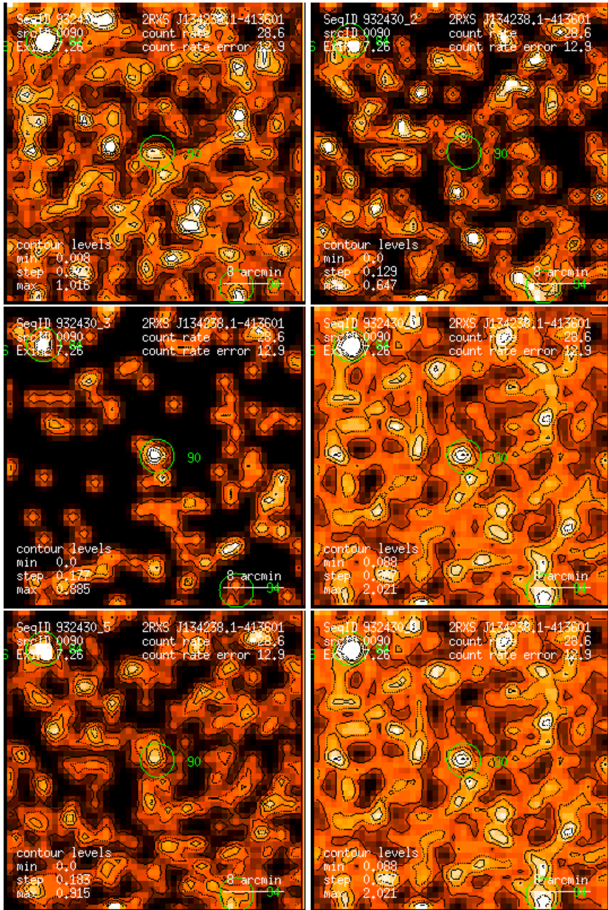
Figure 90: RASS 932430: detection 0090: band rate images, Gaussian filter: (1) PSPC channels 11 – 41, (2) 52 – 90, (3) 91 – 201, (4) 11 – 235, (5) 52 – 201, (6) 11 – 201. Broad band rates in counts/ks. Band rate contour levels in counts/ks/arcmin 2 .
