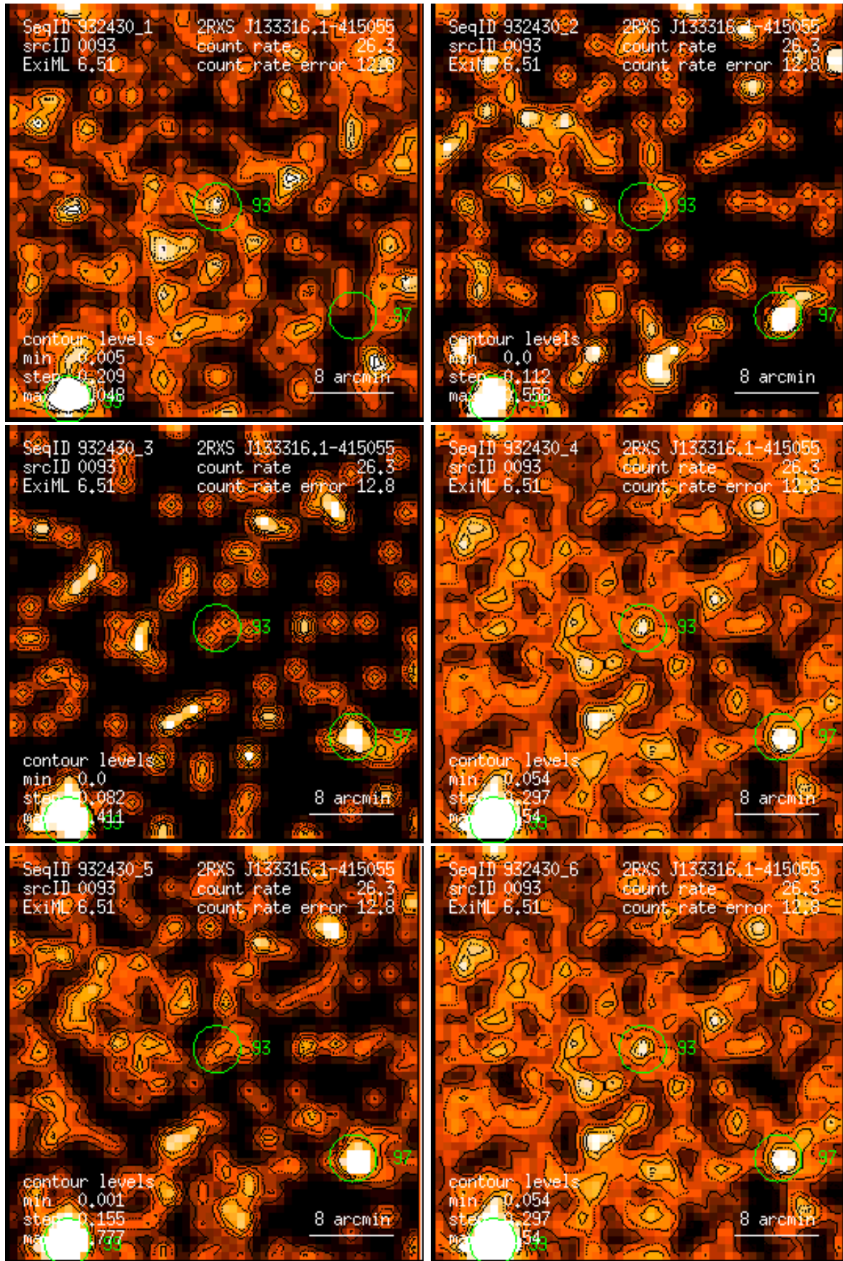
Figure 93: RASS 932430: detection 0093: band rate images, Gaussian filter: (1) PSPC channels 11 – 41, (2) 52 – 90, (3) 91 – 201, (4) 11 – 235, (5) 52 – 201, (6) 11 – 201. Broad band rates in counts/ks. Band rate contour levels in counts/ks/arcmin 2 .
