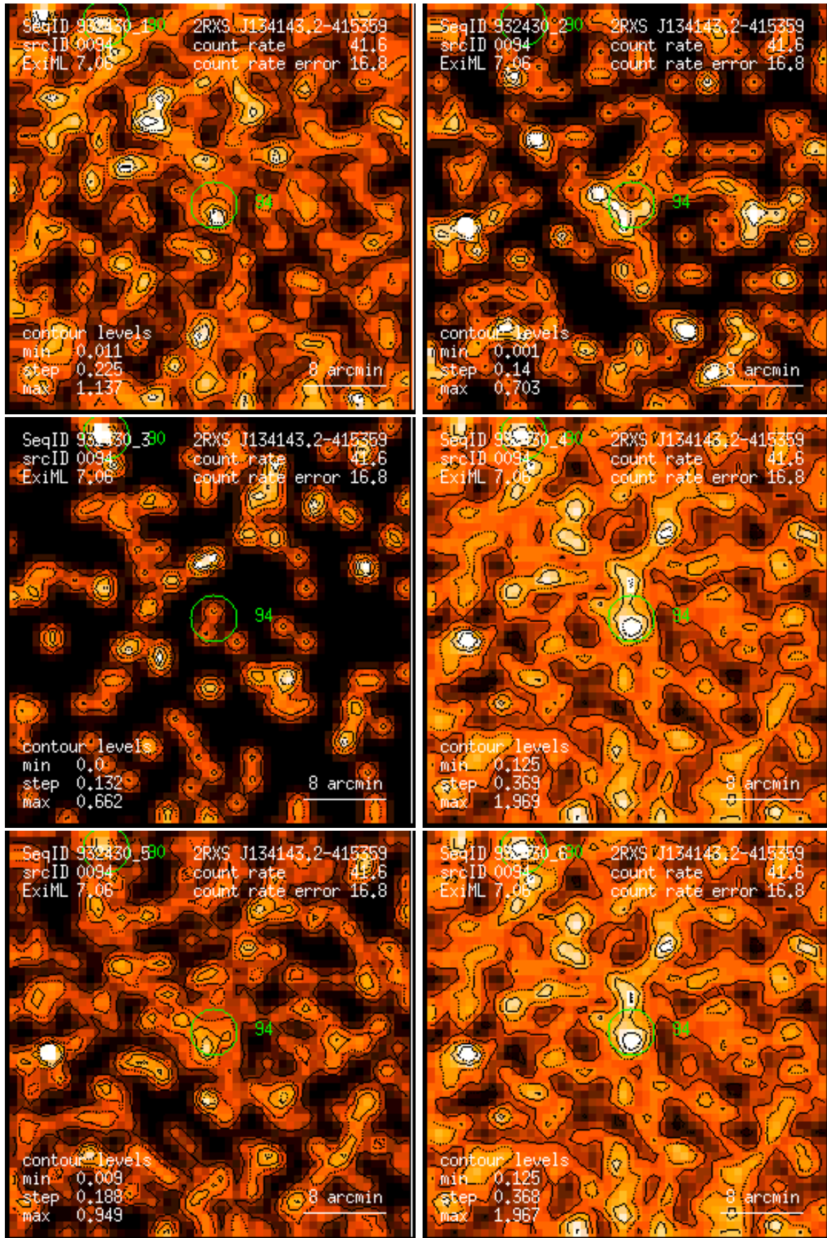
Figure 94: RASS 932430: detection 0094: band rate images, Gaussian filter: (1) PSPC channels 11 – 41, (2) 52 – 90, (3) 91 – 201, (4) 11 – 235, (5) 52 – 201, (6) 11 – 201. Broad band rates in counts/ks. Band rate contour levels in counts/ks/arcmin 2 .
