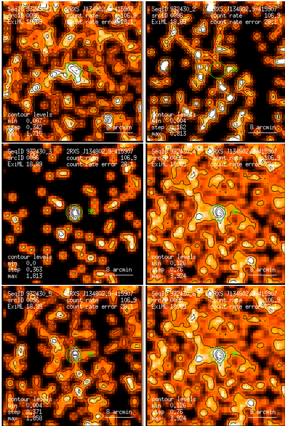
Figure 96: RASS 932430: detection 0096: band rate images, Gaussian filter: (1) PSPC channels 11 – 41, (2) 52 – 90, (3) 91 – 201, (4) 11 – 235, (5) 52 – 201, (6) 11 – 201. Broad band rates in counts/ks. Band rate contour levels in counts/ks/arcmin 2 .
