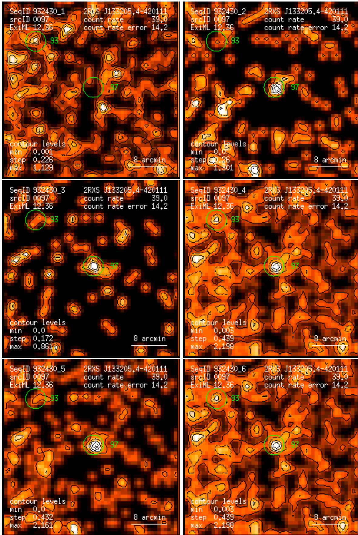
Figure 97: RASS 932430: detection 0097: band rate images, Gaussian filter: (1) PSPC channels 11 – 41, (2) 52 – 90, (3) 91 – 201, (4) 11 – 235, (5) 52 – 201, (6) 11 – 201. Broad band rates in counts/ks. Band rate contour levels in counts/ks/arcmin 2 .
