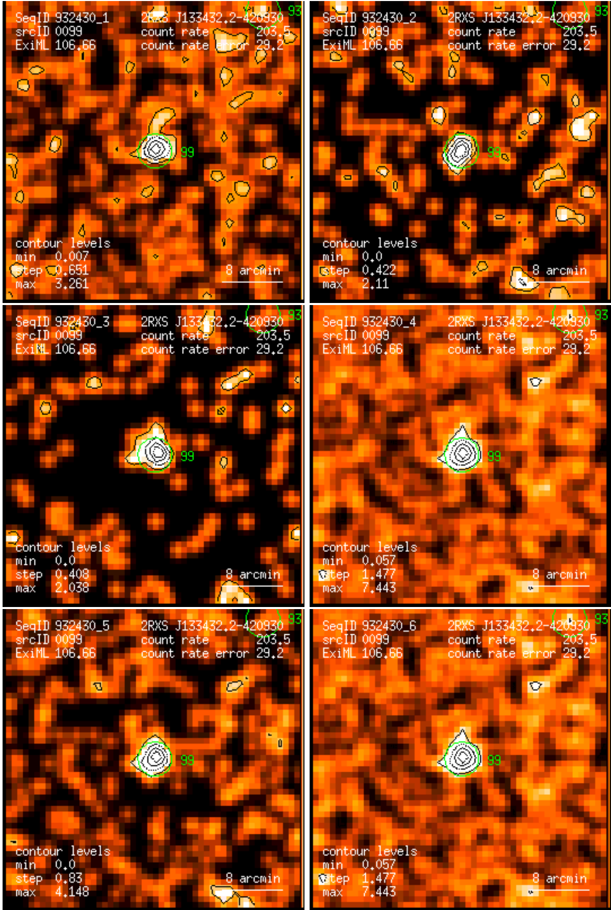
Figure 99: RASS 932430: detection 0099: band rate images, Gaussian filter: (1) PSPC channels 11 – 41, (2) 52 – 90, (3) 91 – 201, (4) 11 – 235, (5) 52 – 201, (6) 11 – 201. Broad band rates in counts/ks. Band rate contour levels in counts/ks/arcmin 2 .
