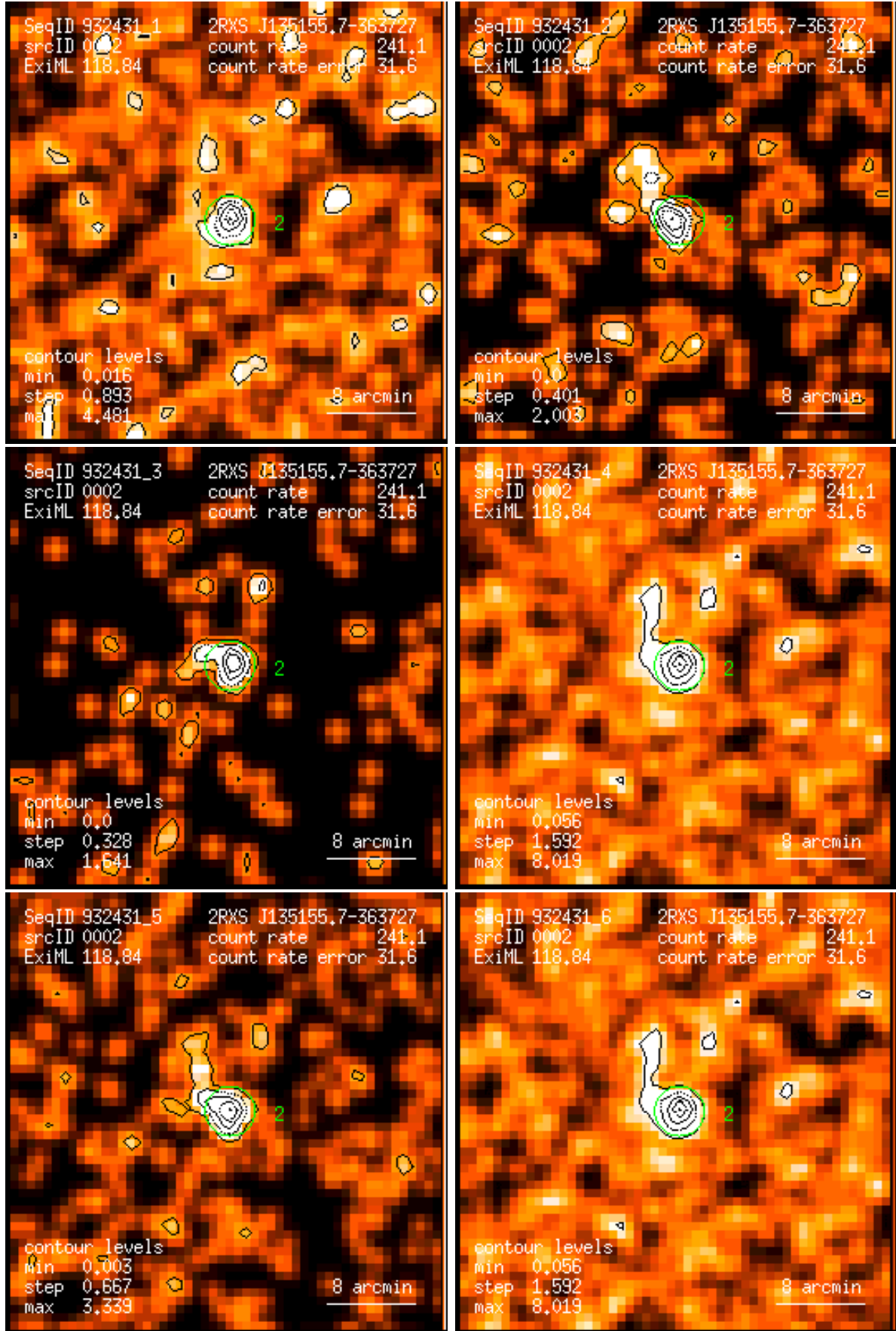
Figure 2: RASS 932431: detection 0002: band rate images, Gaussian filter: (1) PSPC channels 11 – 41, (2) 52 – 90, (3) 91 – 201, (4) 11 – 235, (5) 52 – 201, (6) 11 – 201. Broad band rates in counts/ks. Band rate contour levels in counts/ks/arcmin 2 .
