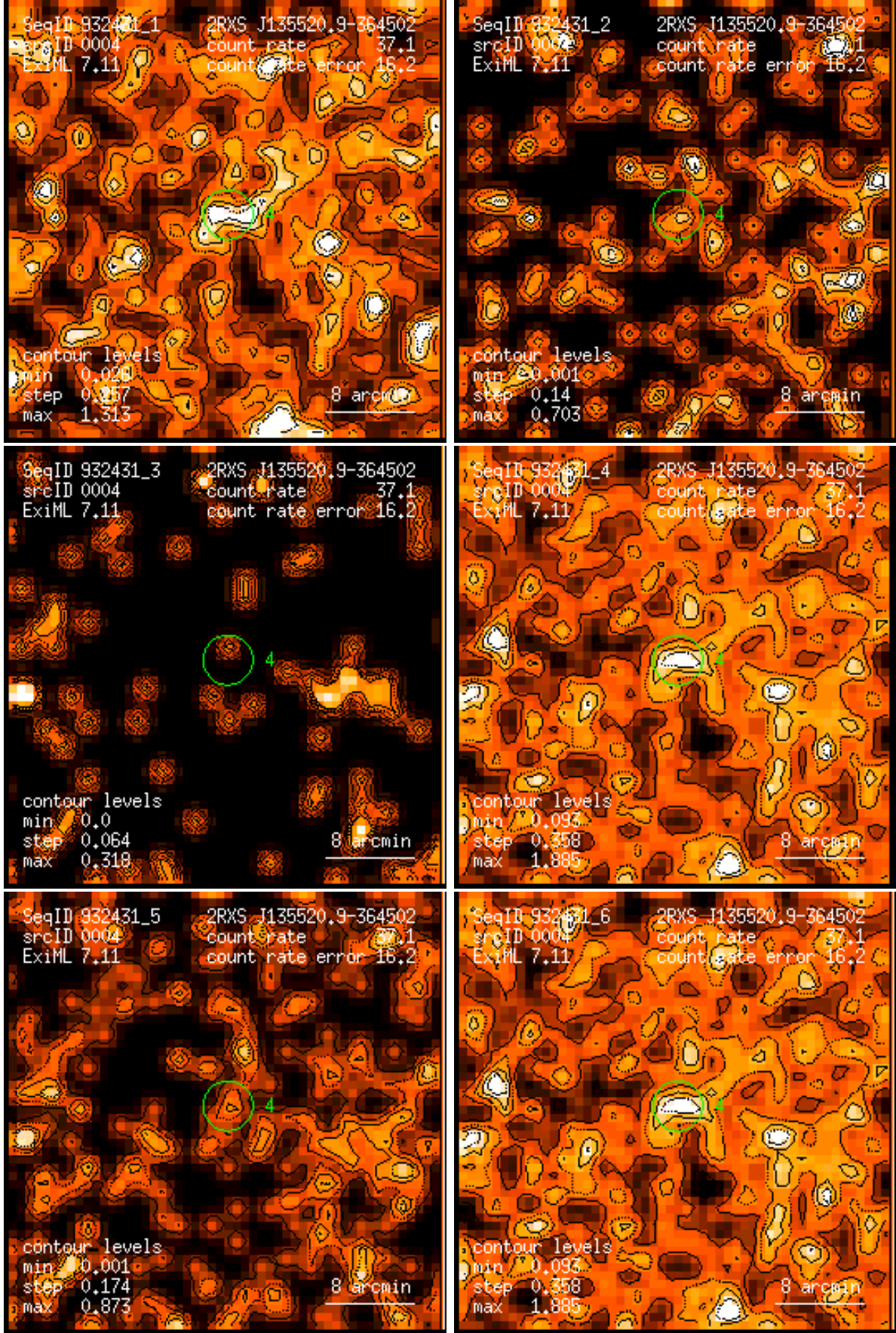
Figure 4: RASS 932431: detection 0004: band rate images, Gaussian filter: (1) PSPC channels 11 – 41, (2) 52 – 90, (3) 91 – 201, (4) 11 – 235, (5) 52 – 201, (6) 11 – 201. Broad band rates in counts/ks. Band rate contour levels in counts/ks/arcmin 2 .
