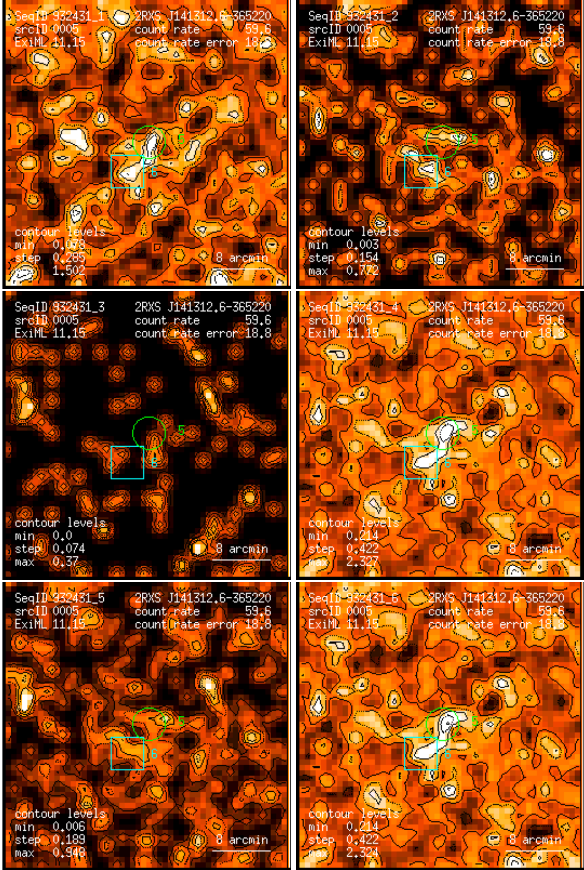
Figure 5: RASS 932431: detection 0005: band rate images, Gaussian filter: (1) PSPC channels 11 – 41, (2) 52 – 90, (3) 91 – 201, (4) 11 – 235, (5) 52 – 201, (6) 11 – 201. Broad band rates in counts/ks. Band rate contour levels in counts/ks/arcmin 2 .
