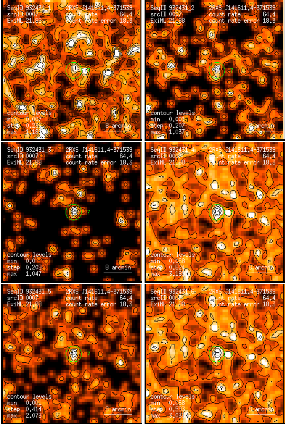
Figure 7: RASS 932431: detection 0007: band rate images, Gaussian filter: (1) PSPC channels 11 – 41, (2) 52 – 90, (3) 91 – 201, (4) 11 – 235, (5) 52 – 201, (6) 11 – 201. Broad band rates in counts/ks. Band rate contour levels in counts/ks/arcmin 2 .
