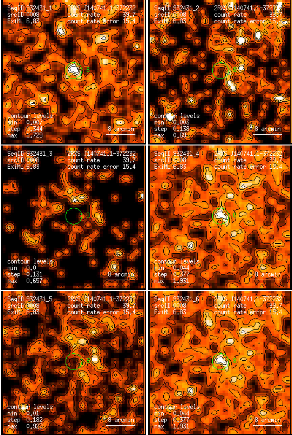
Figure 8: RASS 932431: detection 0008: band rate images, Gaussian filter: (1) PSPC channels 11 – 41, (2) 52 – 90, (3) 91 – 201, (4) 11 – 235, (5) 52 – 201, (6) 11 – 201. Broad band rates in counts/ks. Band rate contour levels in counts/ks/arcmin 2 .
