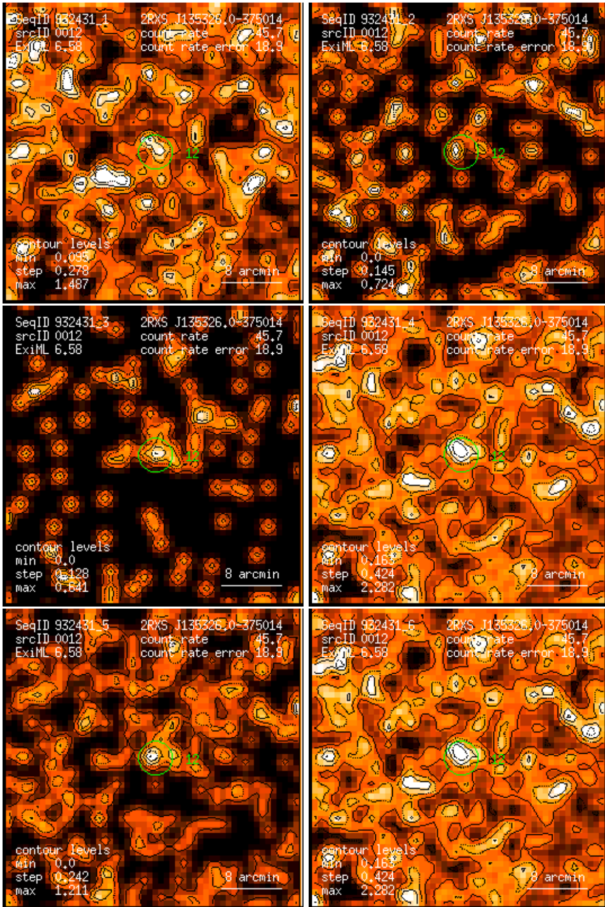
Figure 12: RASS 932431: detection 0012: band rate images, Gaussian filter: (1) PSPC channels 11 – 41, (2) 52 – 90, (3) 91 – 201, (4) 11 – 235, (5) 52 – 201, (6) 11 – 201. Broad band rates in counts/ks. Band rate contour levels in counts/ks/arcmin 2 .
