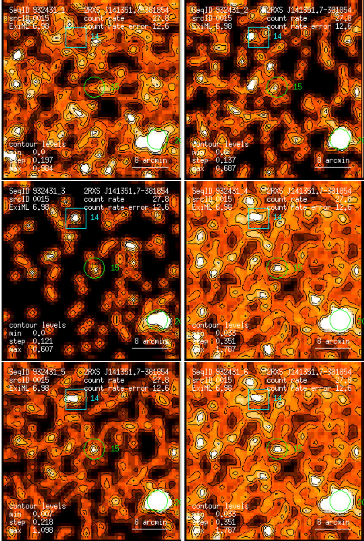
Figure 15: RASS 932431: detection 0015: band rate images, Gaussian filter: (1) PSPC channels 11 – 41, (2) 52 – 90, (3) 91 – 201, (4) 11 – 235, (5) 52 – 201, (6) 11 – 201. Broad band rates in counts/ks. Band rate contour levels in counts/ks/arcmin 2 .
