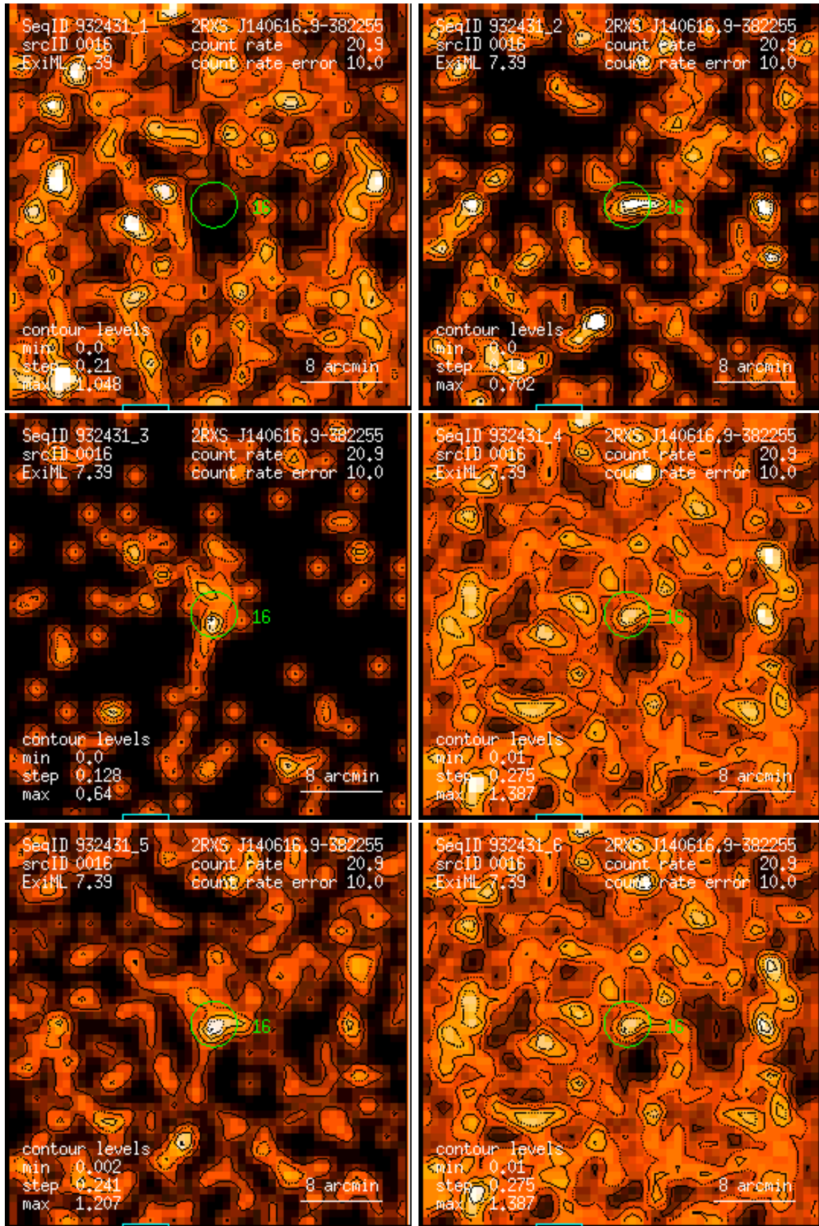
Figure 16: RASS 932431: detection 0016: band rate images, Gaussian filter: (1) PSPC channels 11 – 41, (2) 52 – 90, (3) 91 – 201, (4) 11 – 235, (5) 52 – 201, (6) 11 – 201. Broad band rates in counts/ks. Band rate contour levels in counts/ks/arcmin 2 .
