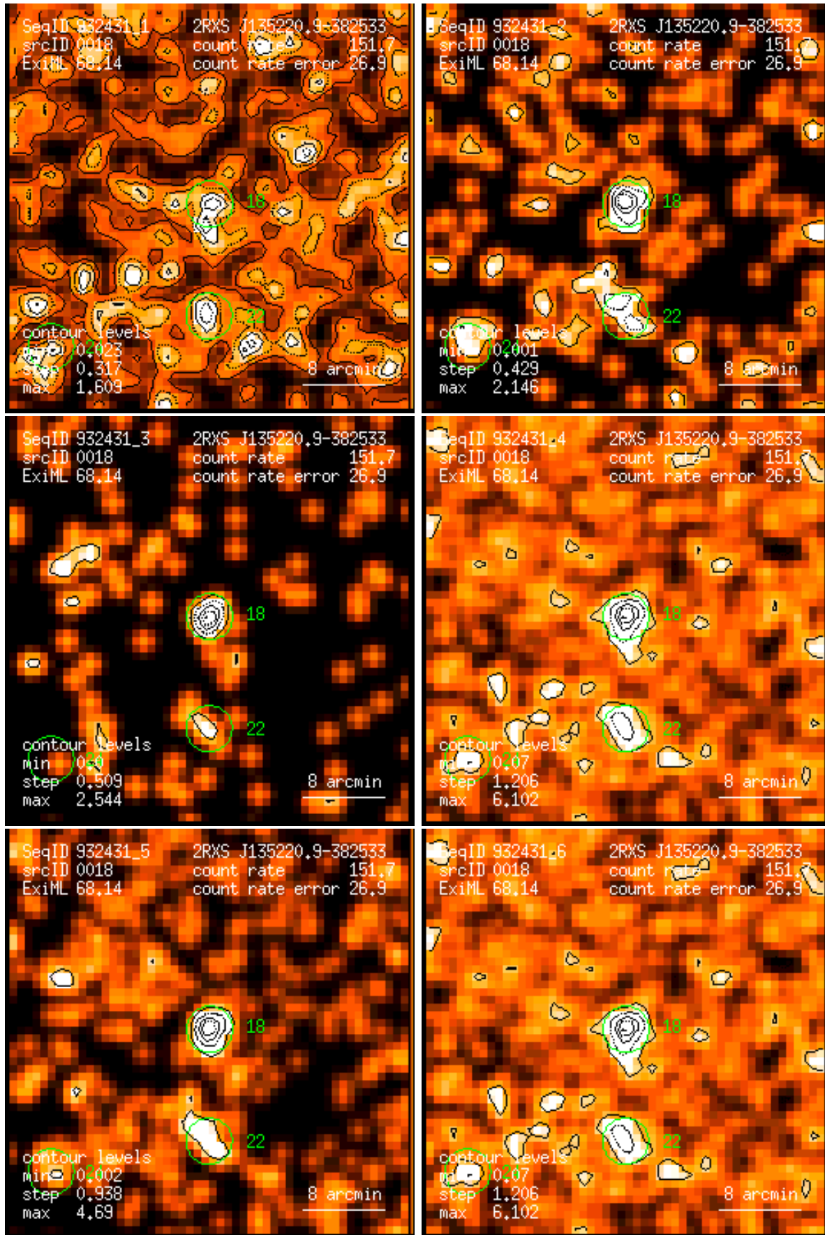
Figure 18: RASS 932431: detection 0018: band rate images, Gaussian filter: (1) PSPC channels 11 – 41, (2) 52 – 90, (3) 91 – 201, (4) 11 – 235, (5) 52 – 201, (6) 11 – 201. Broad band rates in counts/ks. Band rate contour levels in counts/ks/arcmin 2 .
