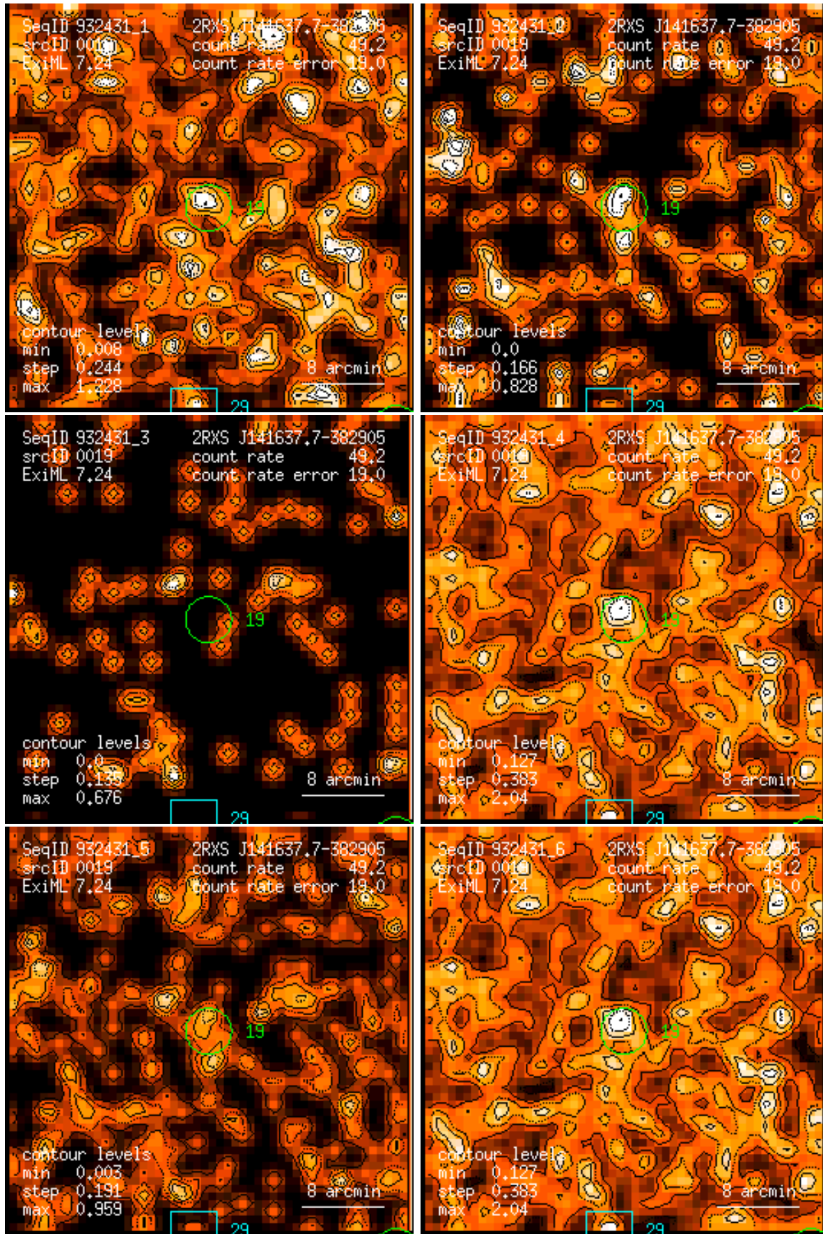
Figure 19: RASS 932431: detection 0019: band rate images, Gaussian filter: (1) PSPC channels 11 – 41, (2) 52 – 90, (3) 91 – 201, (4) 11 – 235, (5) 52 – 201, (6) 11 – 201. Broad band rates in counts/ks. Band rate contour levels in counts/ks/arcmin 2 .
