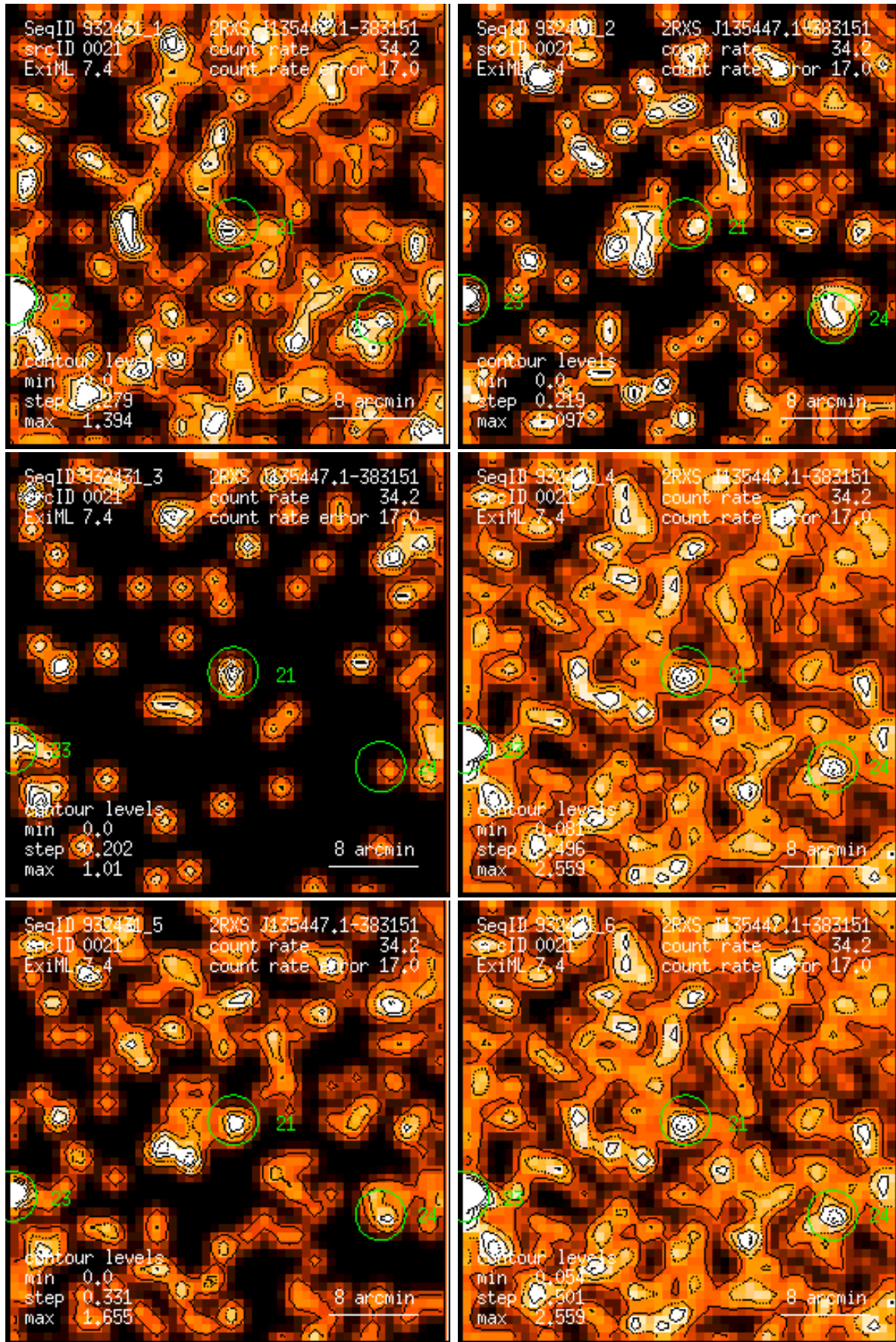
Figure 21: RASS 932431: detection 0021: band rate images, Gaussian filter: (1) PSPC channels 11 – 41, (2) 52 – 90, (3) 91 – 201, (4) 11 – 235, (5) 52 – 201, (6) 11 – 201. Broad band rates in counts/ks. Band rate contour levels in counts/ks/arcmin 2 .
