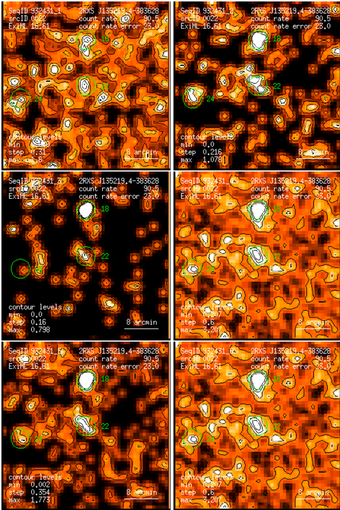
Figure 22: RASS 932431: detection 0022: band rate images, Gaussian filter: (1) PSPC channels 11 – 41, (2) 52 – 90, (3) 91 – 201, (4) 11 – 235, (5) 52 – 201, (6) 11 – 201. Broad band rates in counts/ks. Band rate contour levels in counts/ks/arcmin 2 .
