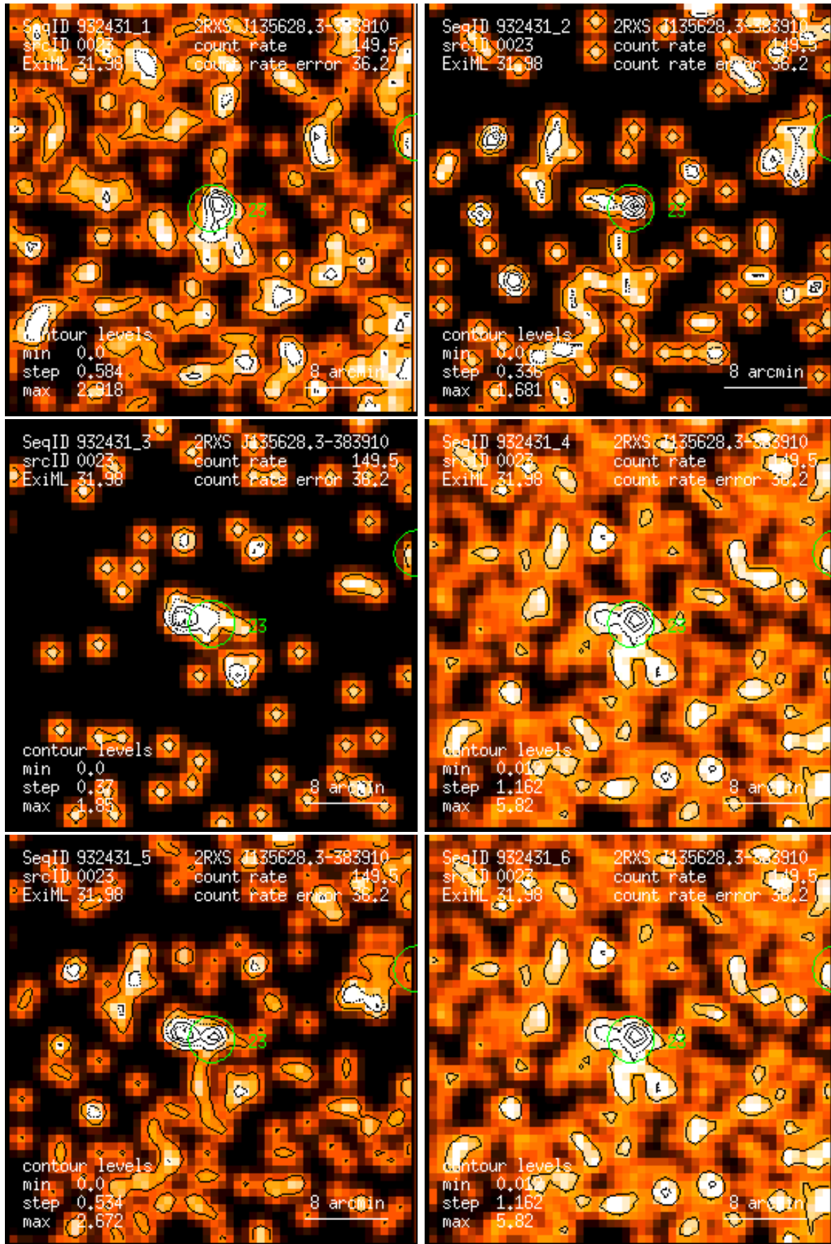
Figure 23: RASS 932431: detection 0023: band rate images, Gaussian filter: (1) PSPC channels 11 – 41, (2) 52 – 90, (3) 91 – 201, (4) 11 – 235, (5) 52 – 201, (6) 11 – 201. Broad band rates in counts/ks. Band rate contour levels in counts/ks/arcmin 2 .
