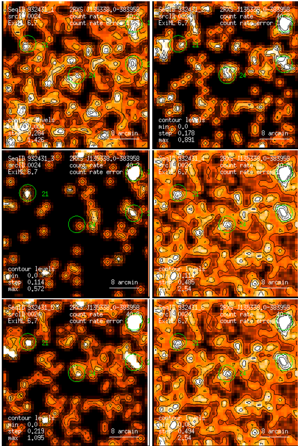
Figure 24: RASS 932431: detection 0024: band rate images, Gaussian filter: (1) PSPC channels 11 – 41, (2) 52 – 90, (3) 91 – 201, (4) 11 – 235, (5) 52 – 201, (6) 11 – 201. Broad band rates in counts/ks. Band rate contour levels in counts/ks/arcmin 2 .
