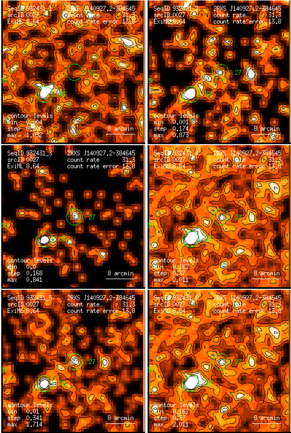
Figure 27: RASS 932431: detection 0027: band rate images, Gaussian filter: (1) PSPC channels 11 – 41, (2) 52 – 90, (3) 91 – 201, (4) 11 – 235, (5) 52 – 201, (6) 11 – 201. Broad band rates in counts/ks. Band rate contour levels in counts/ks/arcmin 2 .
