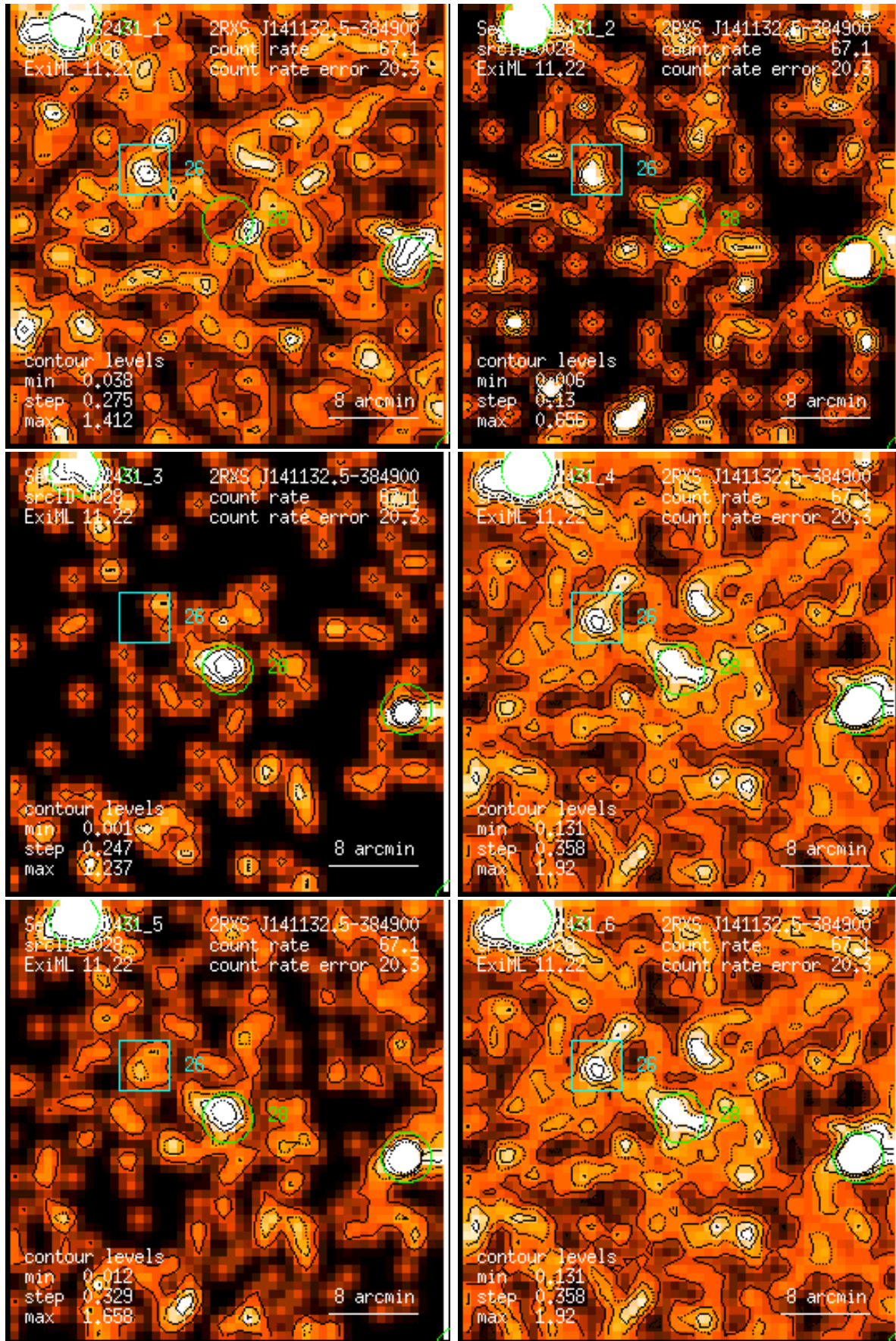
Figure 28: RASS 932431: detection 0028: band rate images, Gaussian filter: (1) PSPC channels 11 – 41, (2) 52 – 90, (3) 91 – 201, (4) 11 – 235, (5) 52 – 201, (6) 11 – 201. Broad band rates in counts/ks. Band rate contour levels in counts/ks/arcmin 2 .
