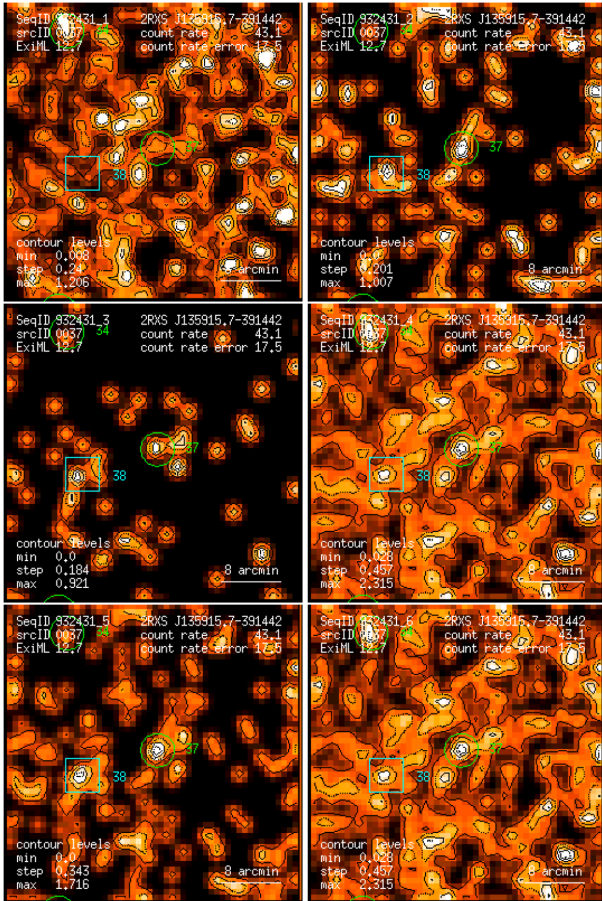
Figure 37: RASS 932431: detection 0037: band rate images, Gaussian filter: (1) PSPC channels 11 – 41, (2) 52 – 90, (3) 91 – 201, (4) 11 – 235, (5) 52 – 201, (6) 11 – 201. Broad band rates in counts/ks. Band rate contour levels in counts/ks/arcmin 2 .
