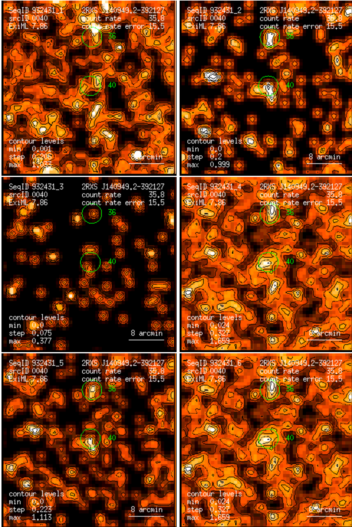
Figure 40: RASS 932431: detection 0040: band rate images, Gaussian filter: (1) PSPC channels 11 – 41, (2) 52 – 90, (3) 91 – 201, (4) 11 – 235, (5) 52 – 201, (6) 11 – 201. Broad band rates in counts/ks. Band rate contour levels in counts/ks/arcmin 2 .
