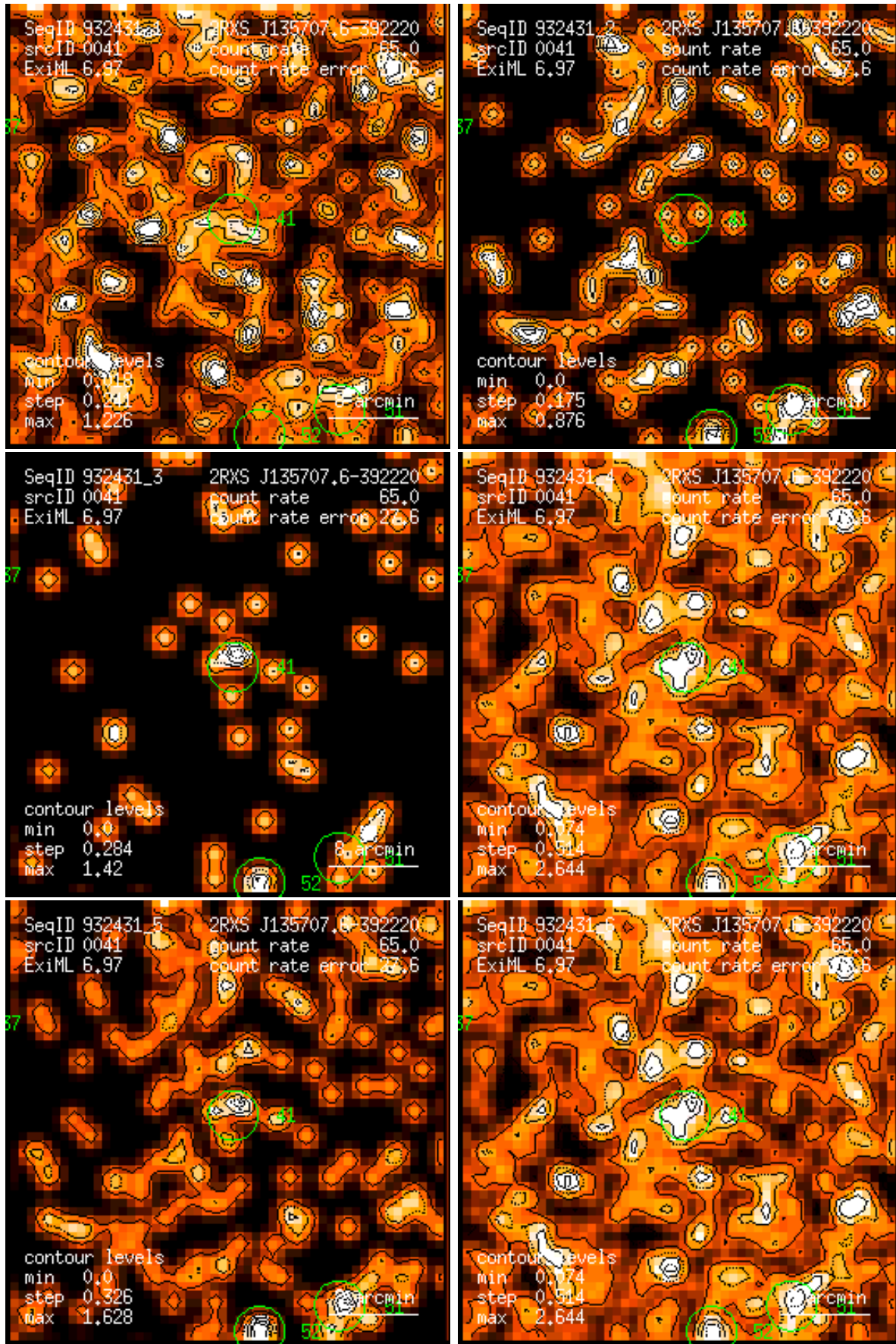
Figure 41: RASS 932431: detection 0041: band rate images, Gaussian filter: (1) PSPC channels 11 – 41, (2) 52 – 90, (3) 91 – 201, (4) 11 – 235, (5) 52 – 201, (6) 11 – 201. Broad band rates in counts/ks. Band rate contour levels in counts/ks/arcmin 2 .
