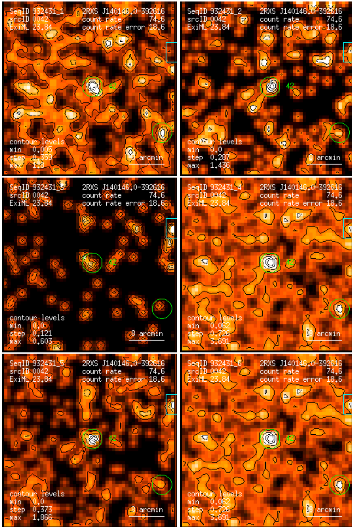
Figure 42: RASS 932431: detection 0042: band rate images, Gaussian filter: (1) PSPC channels 11 – 41, (2) 52 – 90, (3) 91 – 201, (4) 11 – 235, (5) 52 – 201, (6) 11 – 201. Broad band rates in counts/ks. Band rate contour levels in counts/ks/arcmin 2 .
