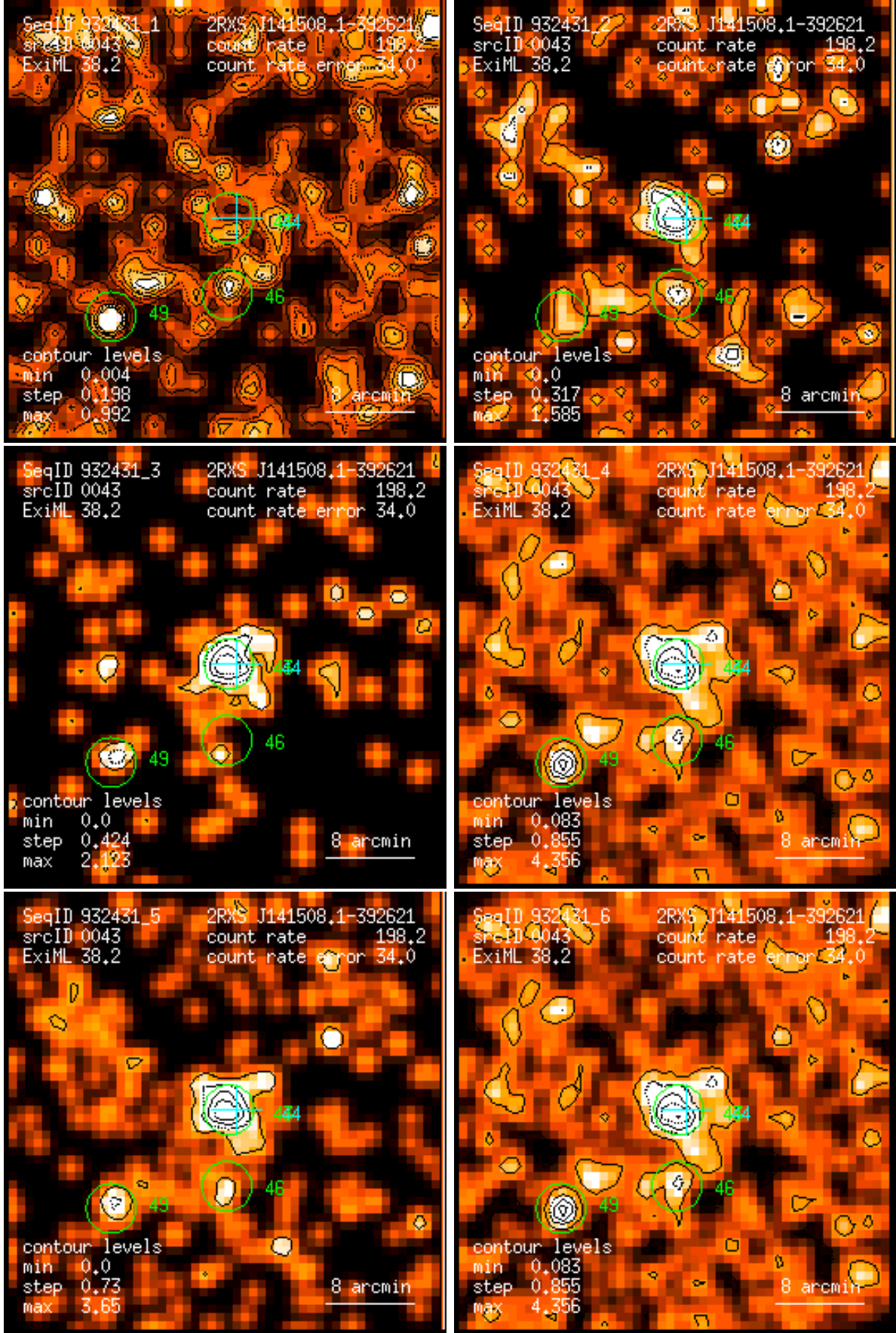
Figure 43: RASS 932431: detection 0043: band rate images, Gaussian filter: (1) PSPC channels 11 – 41, (2) 52 – 90, (3) 91 – 201, (4) 11 – 235, (5) 52 – 201, (6) 11 – 201. Broad band rates in counts/ks. Band rate contour levels in counts/ks/arcmin 2 .
