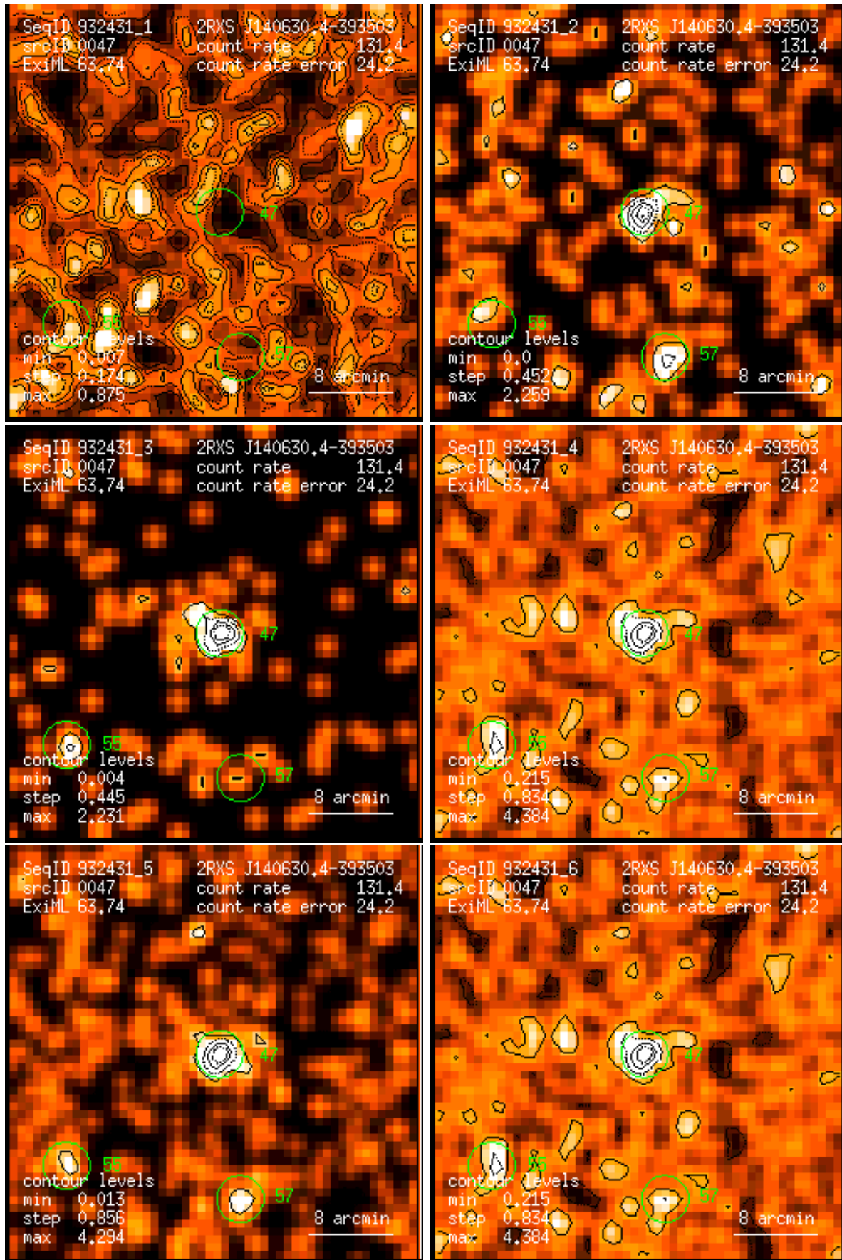
Figure 47: RASS 932431: detection 0047: band rate images, Gaussian filter: (1) PSPC channels 11 – 41, (2) 52 – 90, (3) 91 – 201, (4) 11 – 235, (5) 52 – 201, (6) 11 – 201. Broad band rates in counts/ks. Band rate contour levels in counts/ks/arcmin 2 .
