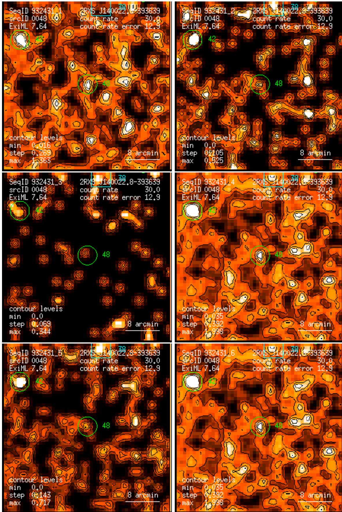
Figure 48: RASS 932431: detection 0048: band rate images, Gaussian filter: (1) PSPC channels 11 – 41, (2) 52 – 90, (3) 91 – 201, (4) 11 – 235, (5) 52 – 201, (6) 11 – 201. Broad band rates in counts/ks. Band rate contour levels in counts/ks/arcmin 2 .
