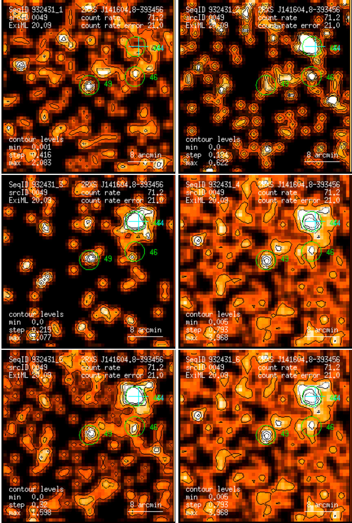
Figure 49: RASS 932431: detection 0049: band rate images, Gaussian filter: (1) PSPC channels 11 – 41, (2) 52 – 90, (3) 91 – 201, (4) 11 – 235, (5) 52 – 201, (6) 11 – 201. Broad band rates in counts/ks. Band rate contour levels in counts/ks/arcmin 2 .
