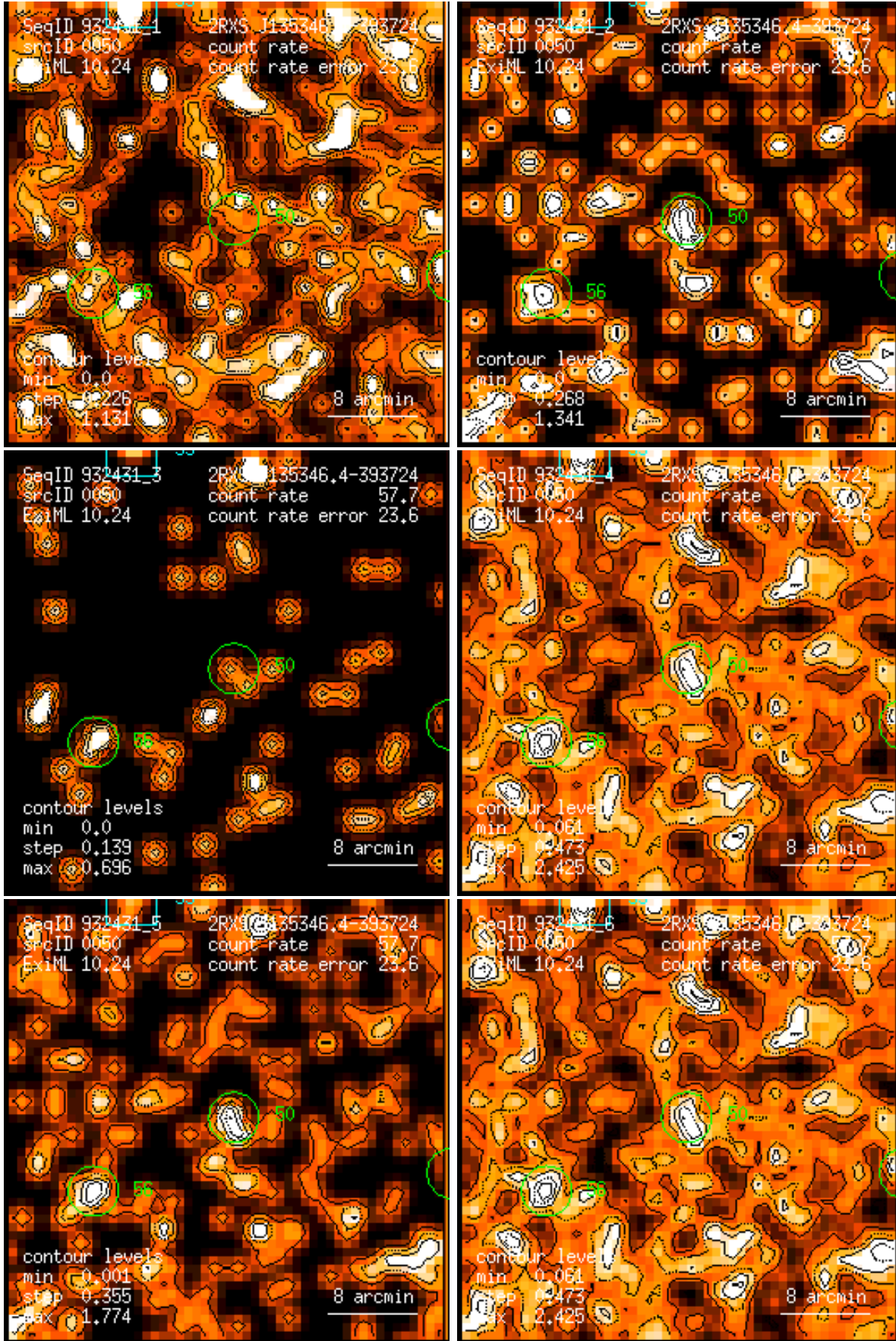
Figure 50: RASS 932431: detection 0050: band rate images, Gaussian filter: (1) PSPC channels 11 – 41, (2) 52 – 90, (3) 91 – 201, (4) 11 – 235, (5) 52 – 201, (6) 11 – 201. Broad band rates in counts/ks. Band rate contour levels in counts/ks/arcmin 2 .
