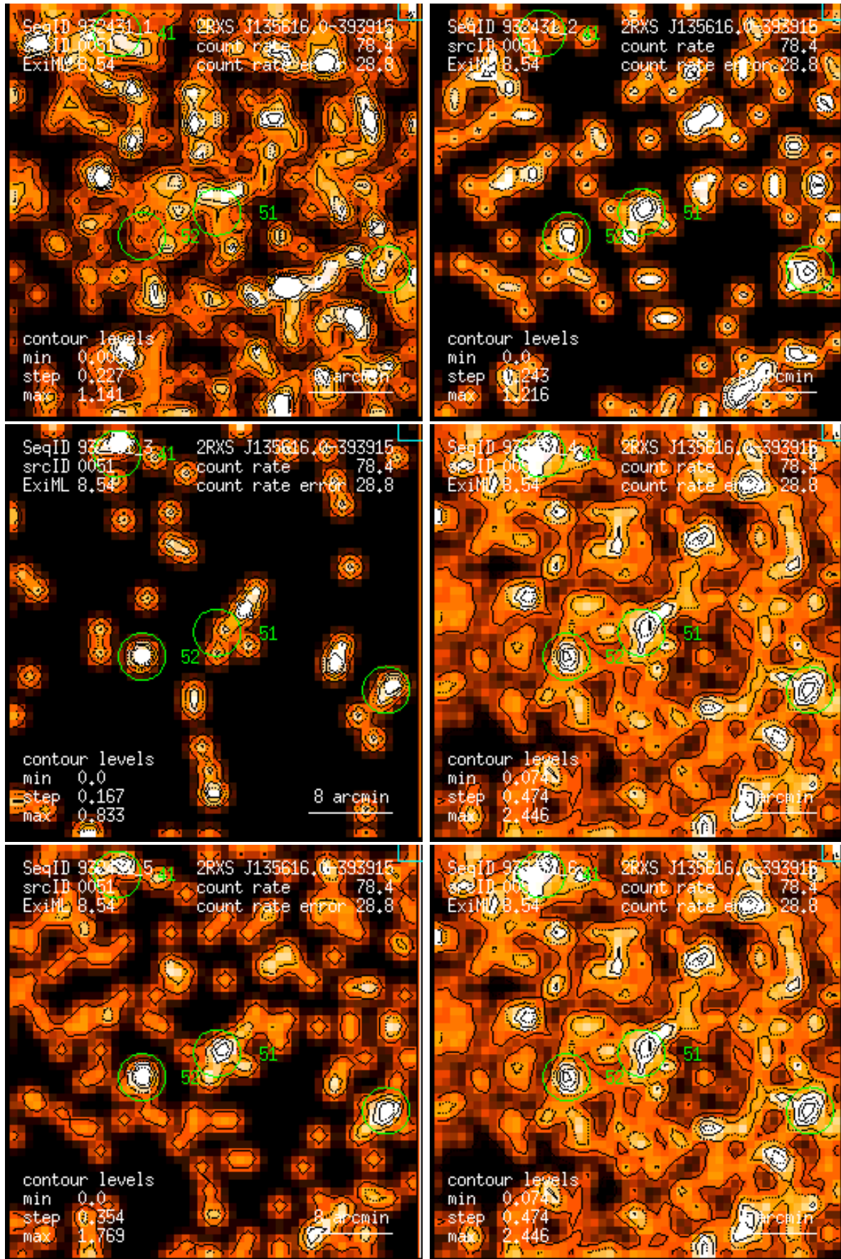
Figure 51: RASS 932431: detection 0051: band rate images, Gaussian filter: (1) PSPC channels 11 – 41, (2) 52 – 90, (3) 91 – 201, (4) 11 – 235, (5) 52 – 201, (6) 11 – 201. Broad band rates in counts/ks. Band rate contour levels in counts/ks/arcmin 2 .
