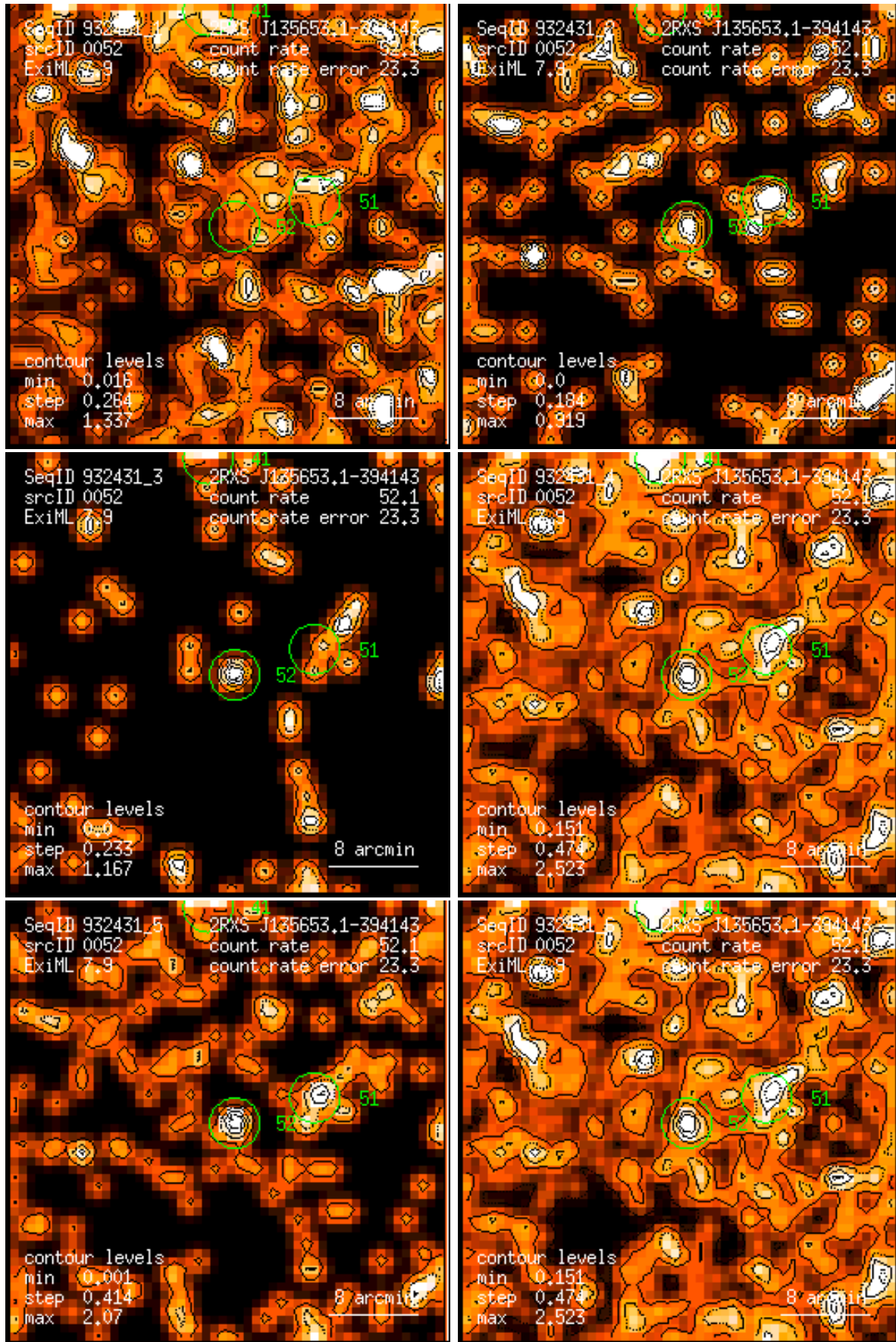
Figure 52: RASS 932431: detection 0052: band rate images, Gaussian filter: (1) PSPC channels 11 – 41, (2) 52 – 90, (3) 91 – 201, (4) 11 – 235, (5) 52 – 201, (6) 11 – 201. Broad band rates in counts/ks. Band rate contour levels in counts/ks/arcmin 2 .
