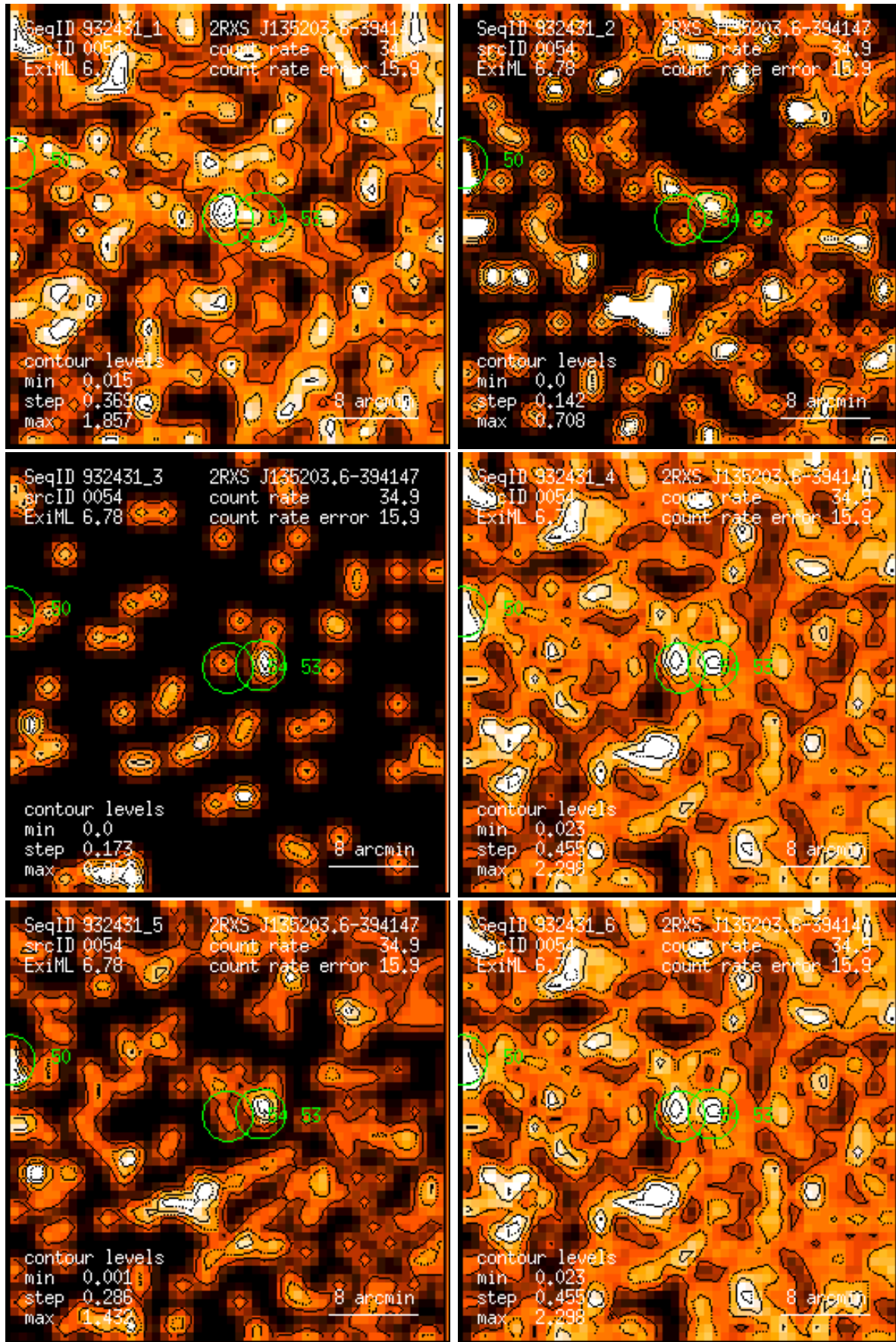
Figure 54: RASS 932431: detection 0054: band rate images, Gaussian filter: (1) PSPC channels 11 – 41, (2) 52 – 90, (3) 91 – 201, (4) 11 – 235, (5) 52 – 201, (6) 11 – 201. Broad band rates in counts/ks. Band rate contour levels in counts/ks/arcmin 2 .
