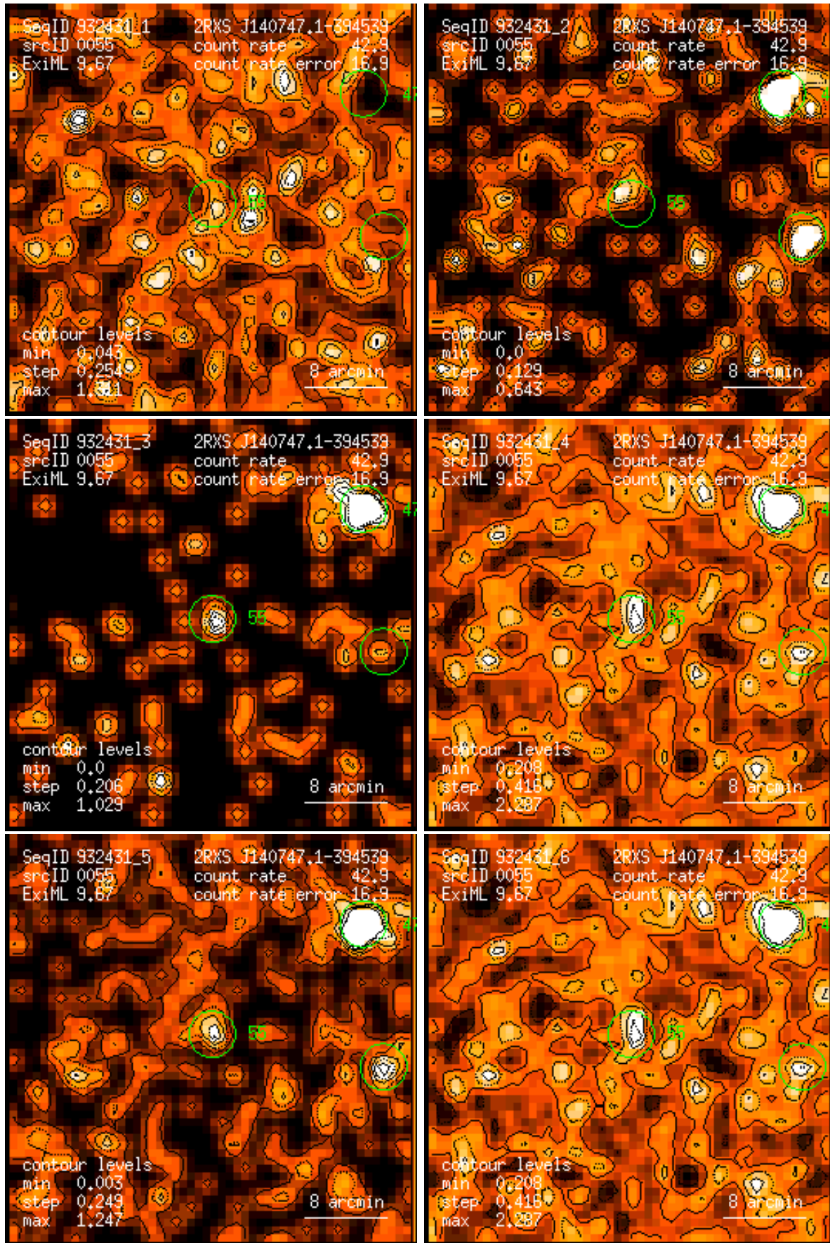
Figure 55: RASS 932431: detection 0055: band rate images, Gaussian filter: (1) PSPC channels 11 – 41, (2) 52 – 90, (3) 91 – 201, (4) 11 – 235, (5) 52 – 201, (6) 11 – 201. Broad band rates in counts/ks. Band rate contour levels in counts/ks/arcmin 2 .
