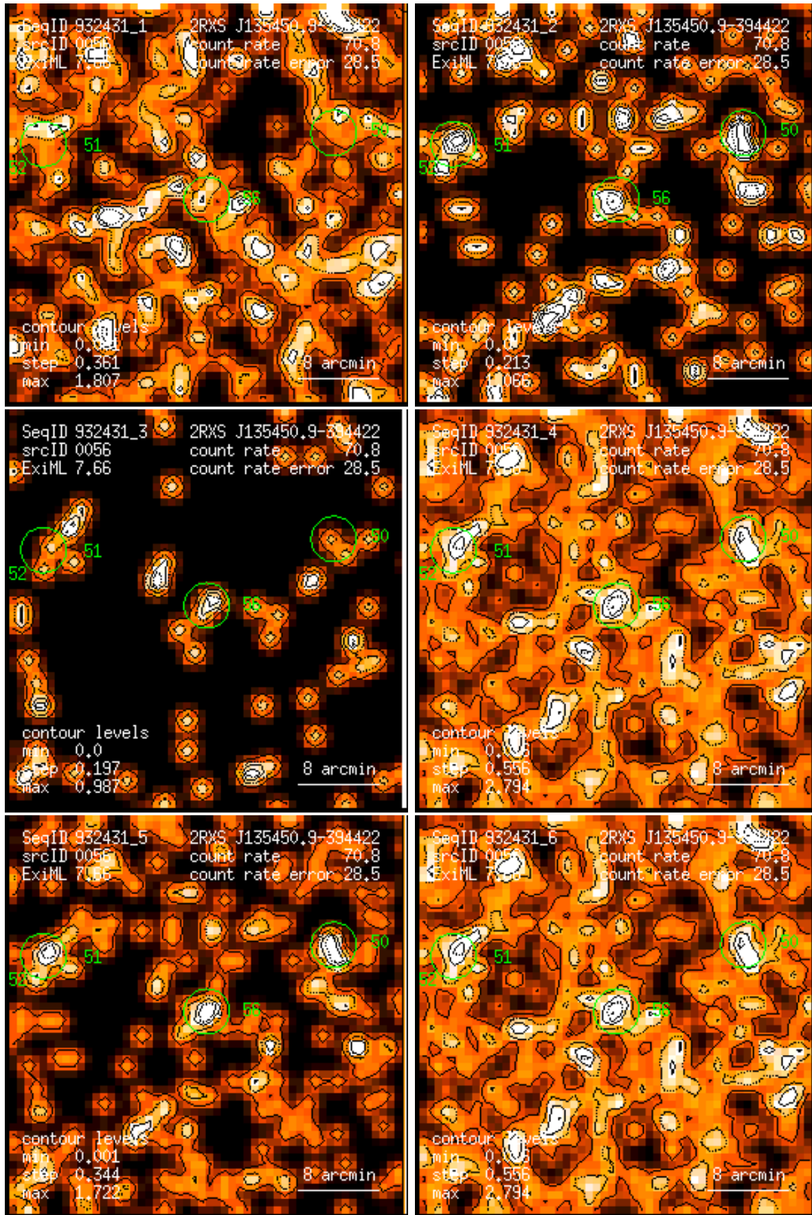
Figure 56: RASS 932431: detection 0056: band rate images, Gaussian filter: (1) PSPC channels 11 – 41, (2) 52 – 90, (3) 91 – 201, (4) 11 – 235, (5) 52 – 201, (6) 11 – 201. Broad band rates in counts/ks. Band rate contour levels in counts/ks/arcmin 2 .
