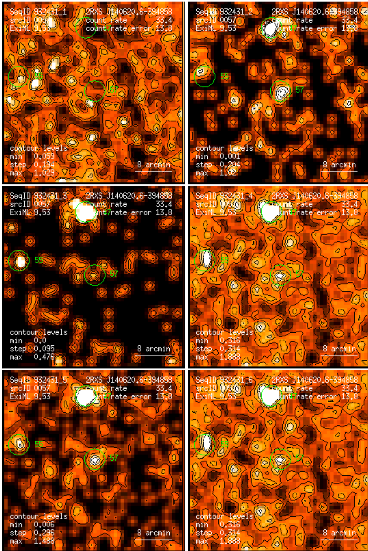
Figure 57: RASS 932431: detection 0057: band rate images, Gaussian filter: (1) PSPC channels 11 – 41, (2) 52 – 90, (3) 91 – 201, (4) 11 – 235, (5) 52 – 201, (6) 11 – 201. Broad band rates in counts/ks. Band rate contour levels in counts/ks/arcmin 2 .
