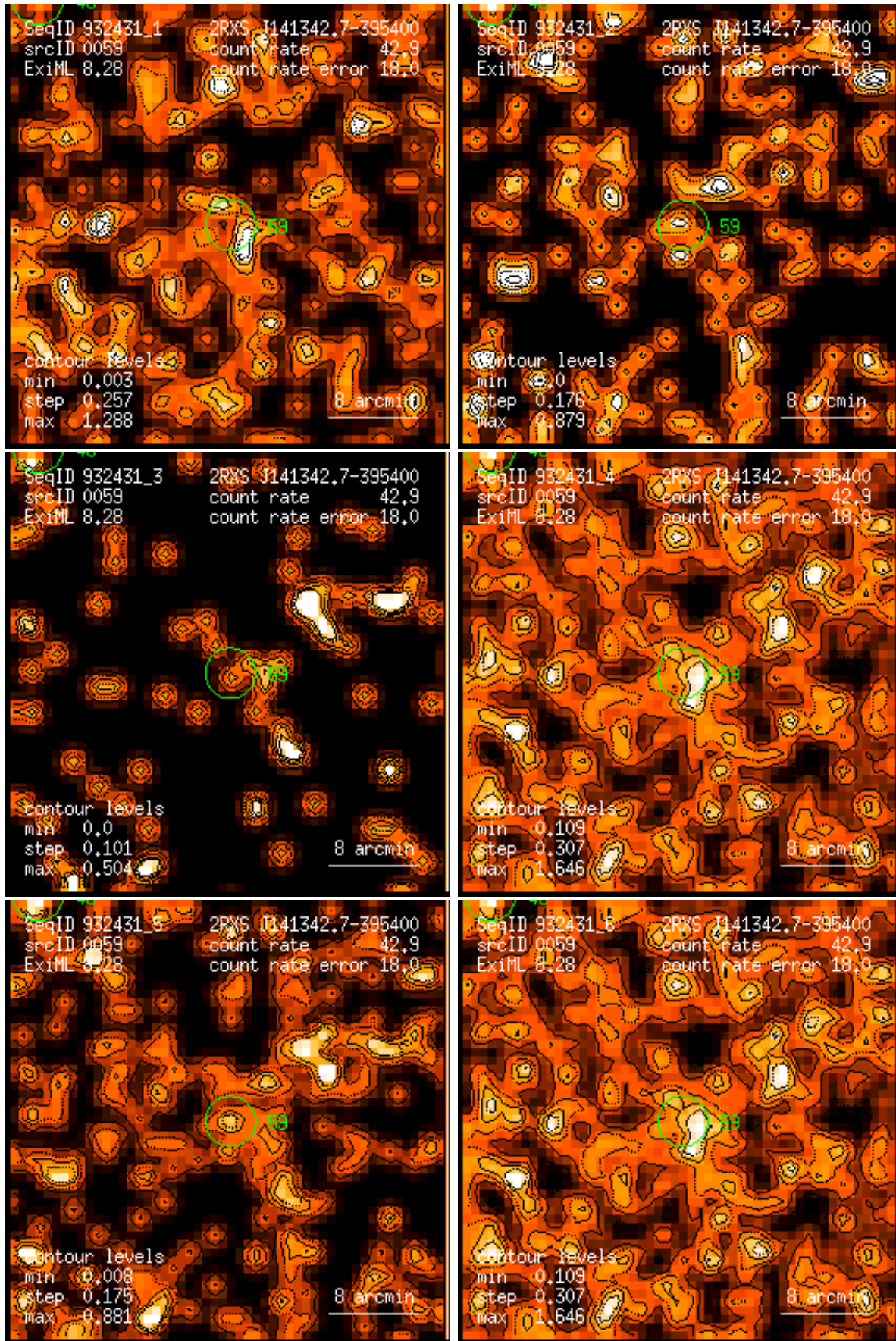
Figure 59: RASS 932431: detection 0059: band rate images, Gaussian filter: (1) PSPC channels 11 – 41, (2) 52 – 90, (3) 91 – 201, (4) 11 – 235, (5) 52 – 201, (6) 11 – 201. Broad band rates in counts/ks. Band rate contour levels in counts/ks/arcmin 2 .
