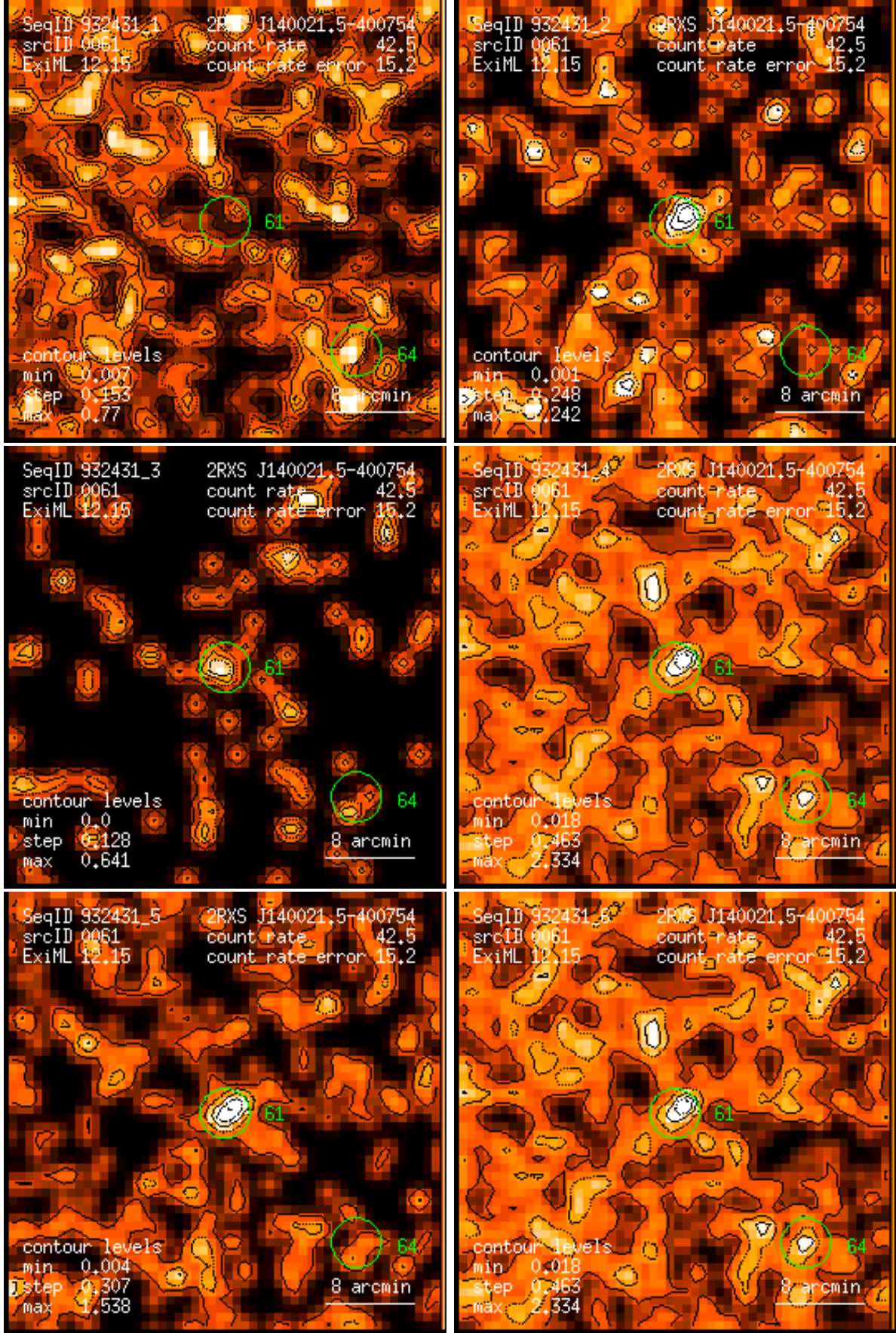
Figure 61: RASS 932431: detection 0061: band rate images, Gaussian filter: (1) PSPC channels 11 – 41, (2) 52 – 90, (3) 91 – 201, (4) 11 – 235, (5) 52 – 201, (6) 11 – 201. Broad band rates in counts/ks. Band rate contour levels in counts/ks/arcmin 2 .
