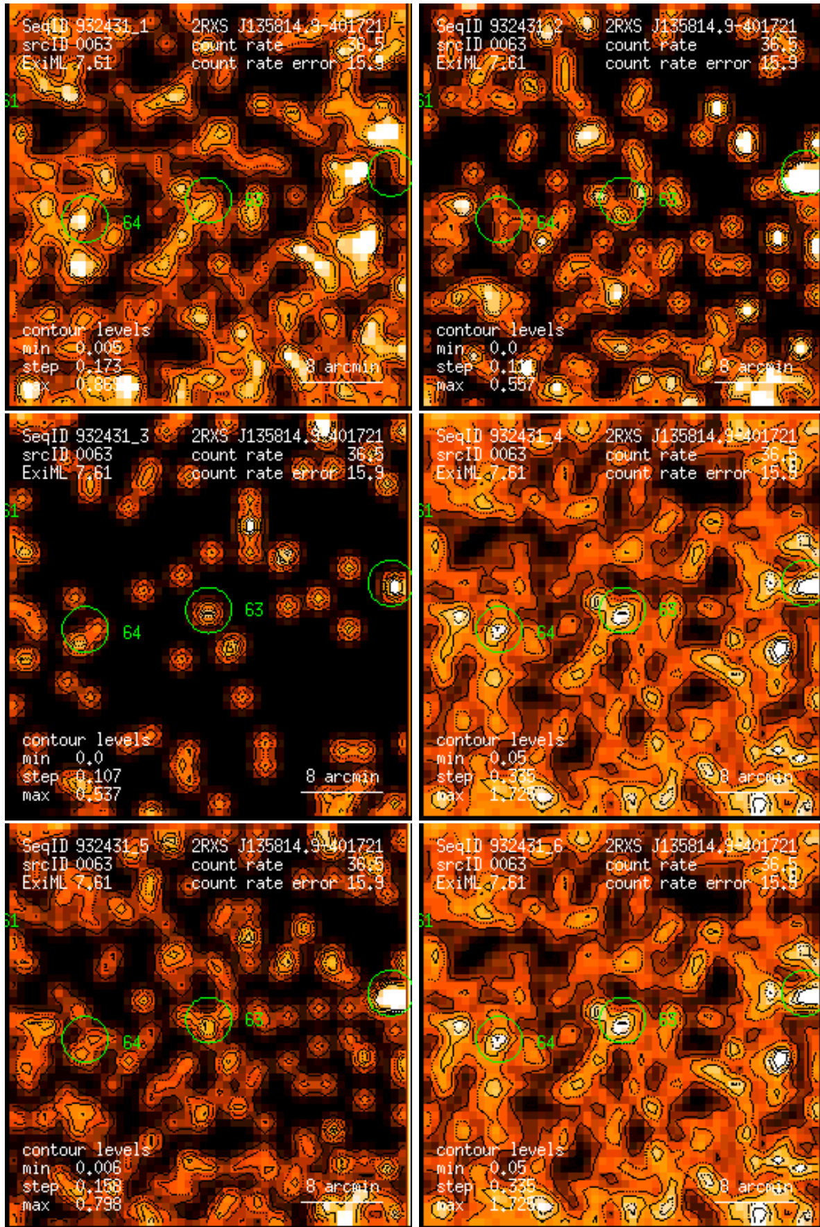
Figure 63: RASS 932431: detection 0063: band rate images, Gaussian filter: (1) PSPC channels 11 – 41, (2) 52 – 90, (3) 91 – 201, (4) 11 – 235, (5) 52 – 201, (6) 11 – 201. Broad band rates in counts/ks. Band rate contour levels in counts/ks/arcmin 2 .
