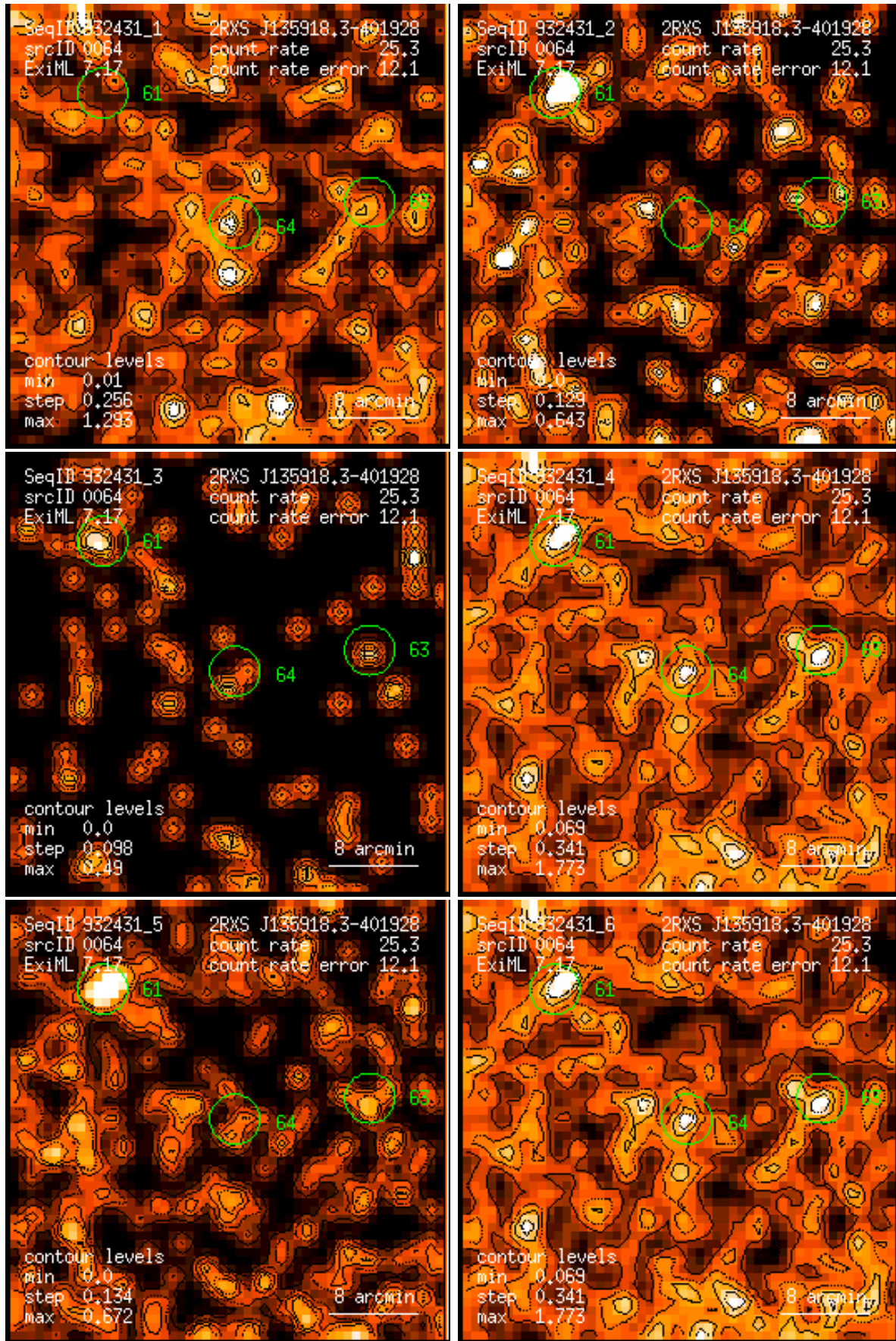
Figure 64: RASS 932431: detection 0064: band rate images, Gaussian filter: (1) PSPC channels 11 – 41, (2) 52 – 90, (3) 91 – 201, (4) 11 – 235, (5) 52 – 201, (6) 11 – 201. Broad band rates in counts/ks. Band rate contour levels in counts/ks/arcmin 2 .
