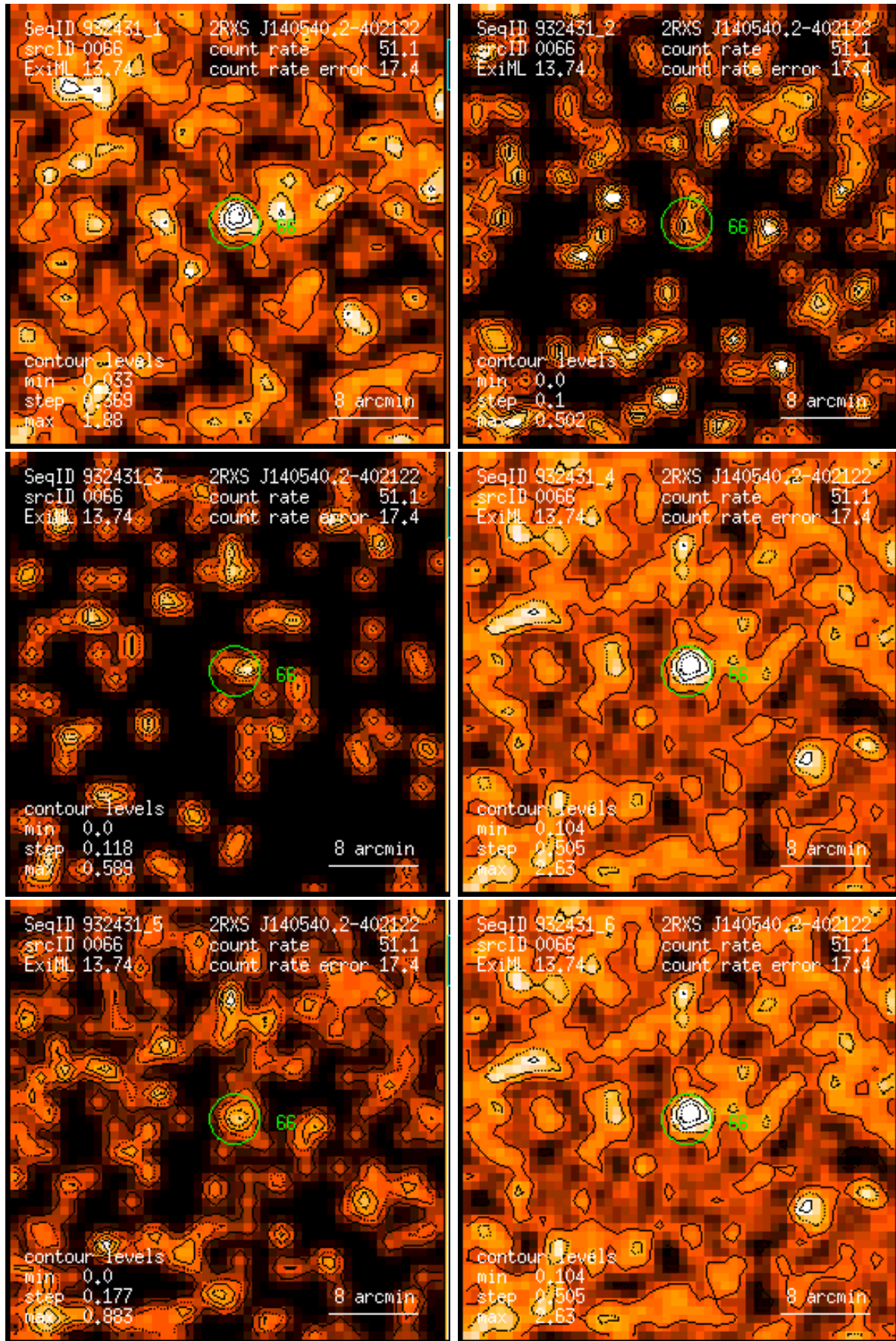
Figure 66: RASS 932431: detection 0066: band rate images, Gaussian filter: (1) PSPC channels 11 – 41, (2) 52 – 90, (3) 91 – 201, (4) 11 – 235, (5) 52 – 201, (6) 11 – 201. Broad band rates in counts/ks. Band rate contour levels in counts/ks/arcmin 2 .
