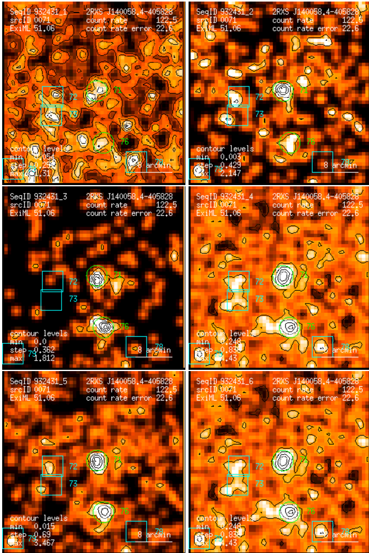
Figure 71: RASS 932431: detection 0071: band rate images, Gaussian filter: (1) PSPC channels 11 – 41, (2) 52 – 90, (3) 91 – 201, (4) 11 – 235, (5) 52 – 201, (6) 11 – 201. Broad band rates in counts/ks. Band rate contour levels in counts/ks/arcmin 2 .
