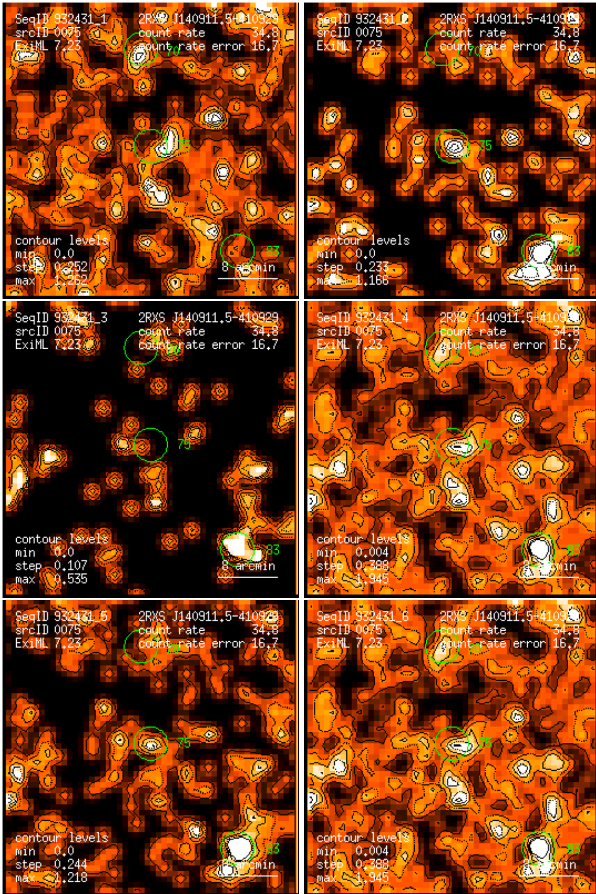
Figure 75: RASS 932431: detection 0075: band rate images, Gaussian filter: (1) PSPC channels 11 – 41, (2) 52 – 90, (3) 91 – 201, (4) 11 – 235, (5) 52 – 201, (6) 11 – 201. Broad band rates in counts/ks. Band rate contour levels in counts/ks/arcmin 2 .
