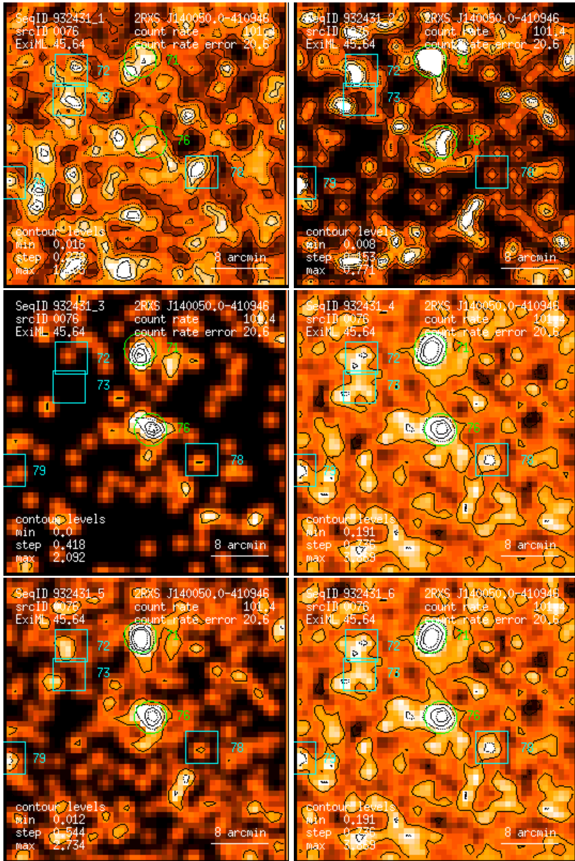
Figure 76: RASS 932431: detection 0076: band rate images, Gaussian filter: (1) PSPC channels 11 – 41, (2) 52 – 90, (3) 91 – 201, (4) 11 – 235, (5) 52 – 201, (6) 11 – 201. Broad band rates in counts/ks. Band rate contour levels in counts/ks/arcmin 2 .
