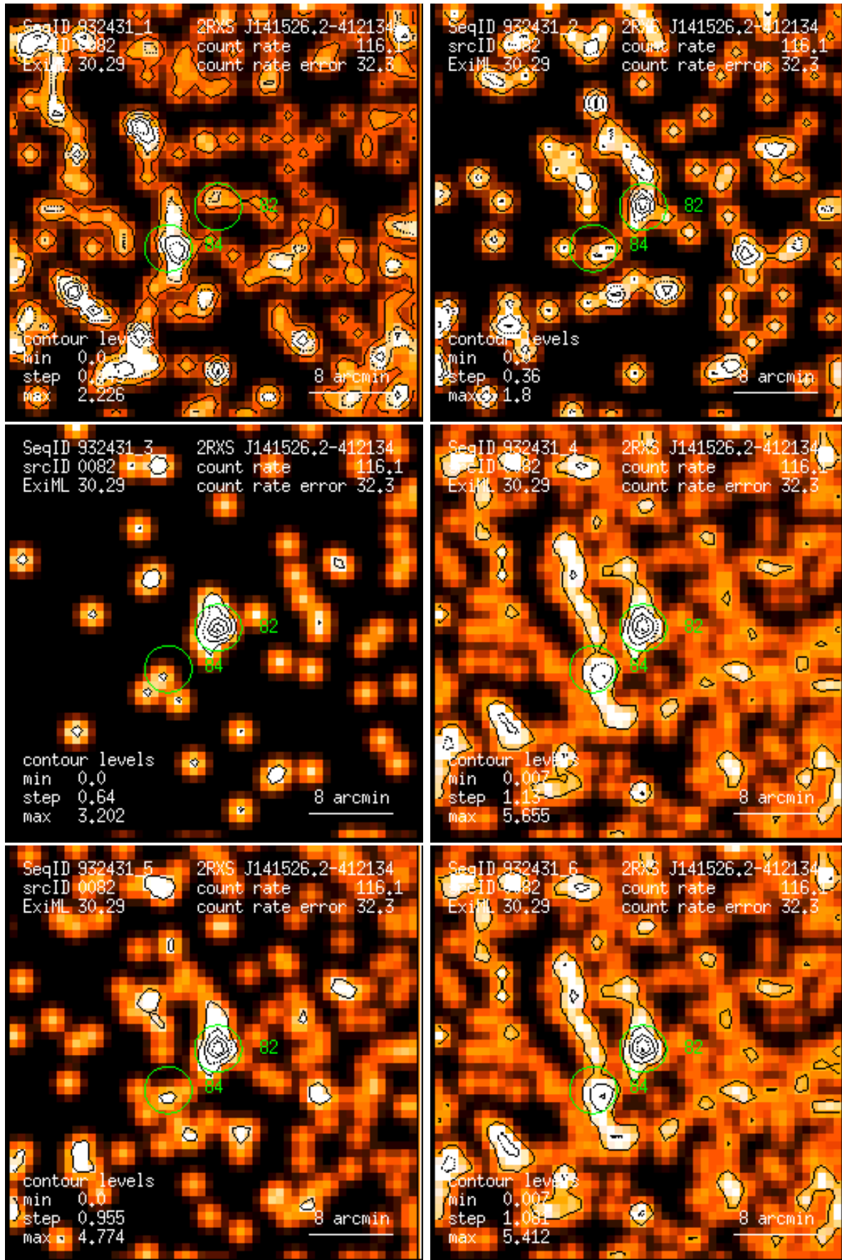
Figure 82: RASS 932431: detection 0082: band rate images, Gaussian filter: (1) PSPC channels 11 – 41, (2) 52 – 90, (3) 91 – 201, (4) 11 – 235, (5) 52 – 201, (6) 11 – 201. Broad band rates in counts/ks. Band rate contour levels in counts/ks/arcmin 2 .
