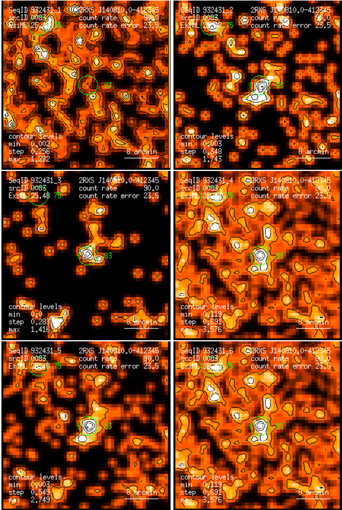
Figure 83: RASS 932431: detection 0083: band rate images, Gaussian filter: (1) PSPC channels 11 – 41, (2) 52 – 90, (3) 91 – 201, (4) 11 – 235, (5) 52 – 201, (6) 11 – 201. Broad band rates in counts/ks. Band rate contour levels in counts/ks/arcmin 2 .
