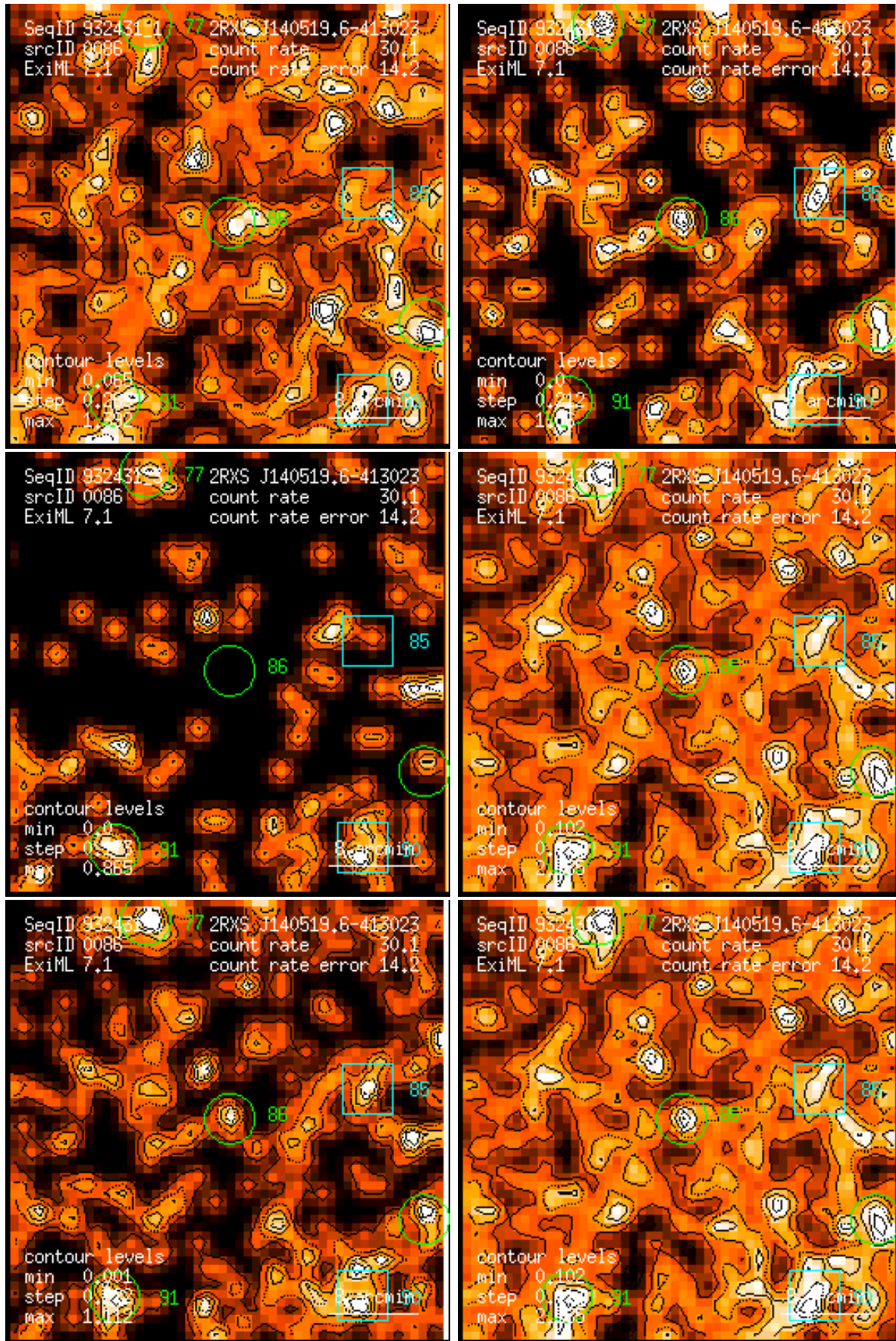
Figure 86: RASS 932431: detection 0086: band rate images, Gaussian filter: (1) PSPC channels 11 – 41, (2) 52 – 90, (3) 91 – 201, (4) 11 – 235, (5) 52 – 201, (6) 11 – 201. Broad band rates in counts/ks. Band rate contour levels in counts/ks/arcmin 2 .
