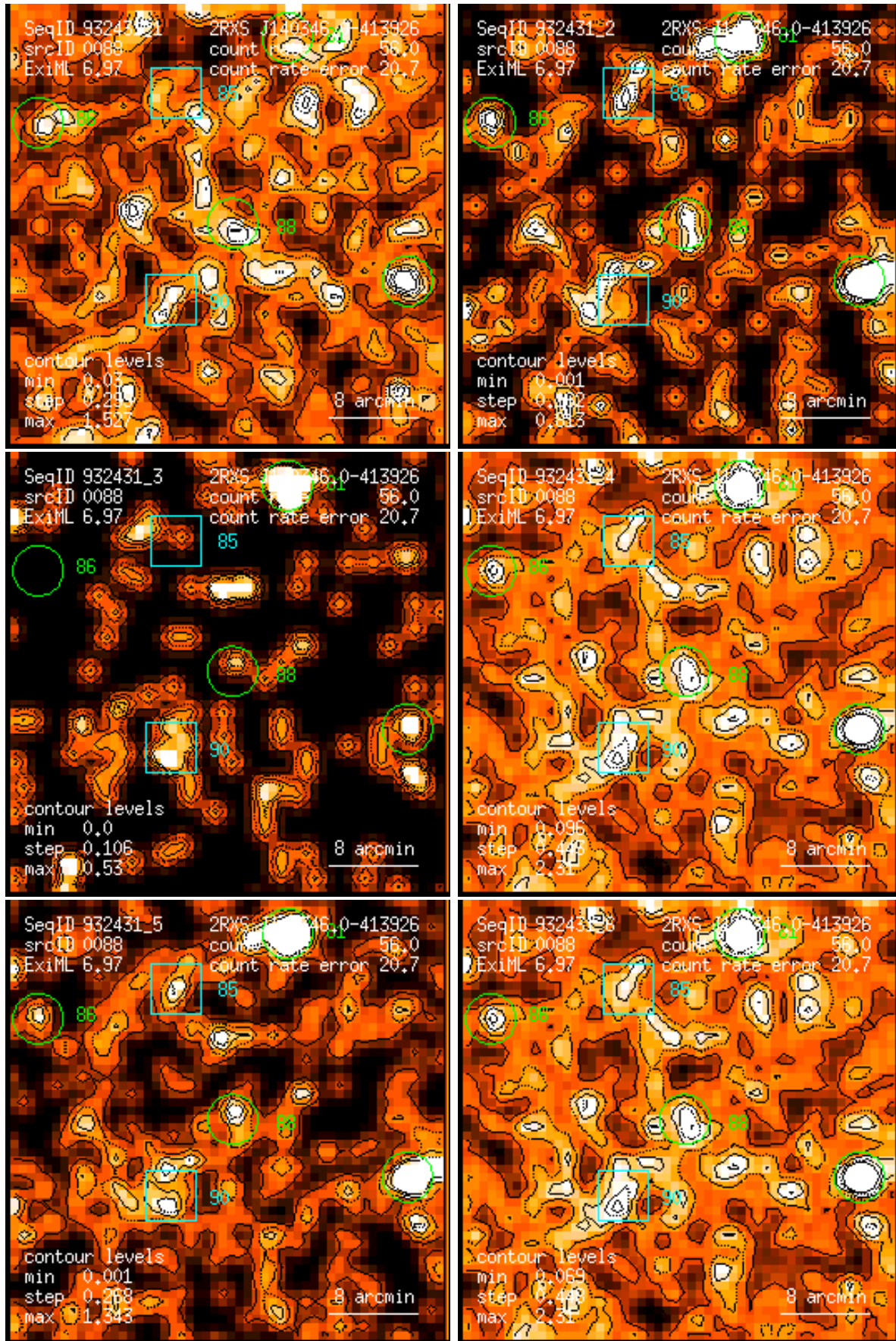
Figure 88: RASS 932431: detection 0088: band rate images, Gaussian filter: (1) PSPC channels 11 – 41, (2) 52 – 90, (3) 91 – 201, (4) 11 – 235, (5) 52 – 201, (6) 11 – 201. Broad band rates in counts/ks. Band rate contour levels in counts/ks/arcmin 2 .
