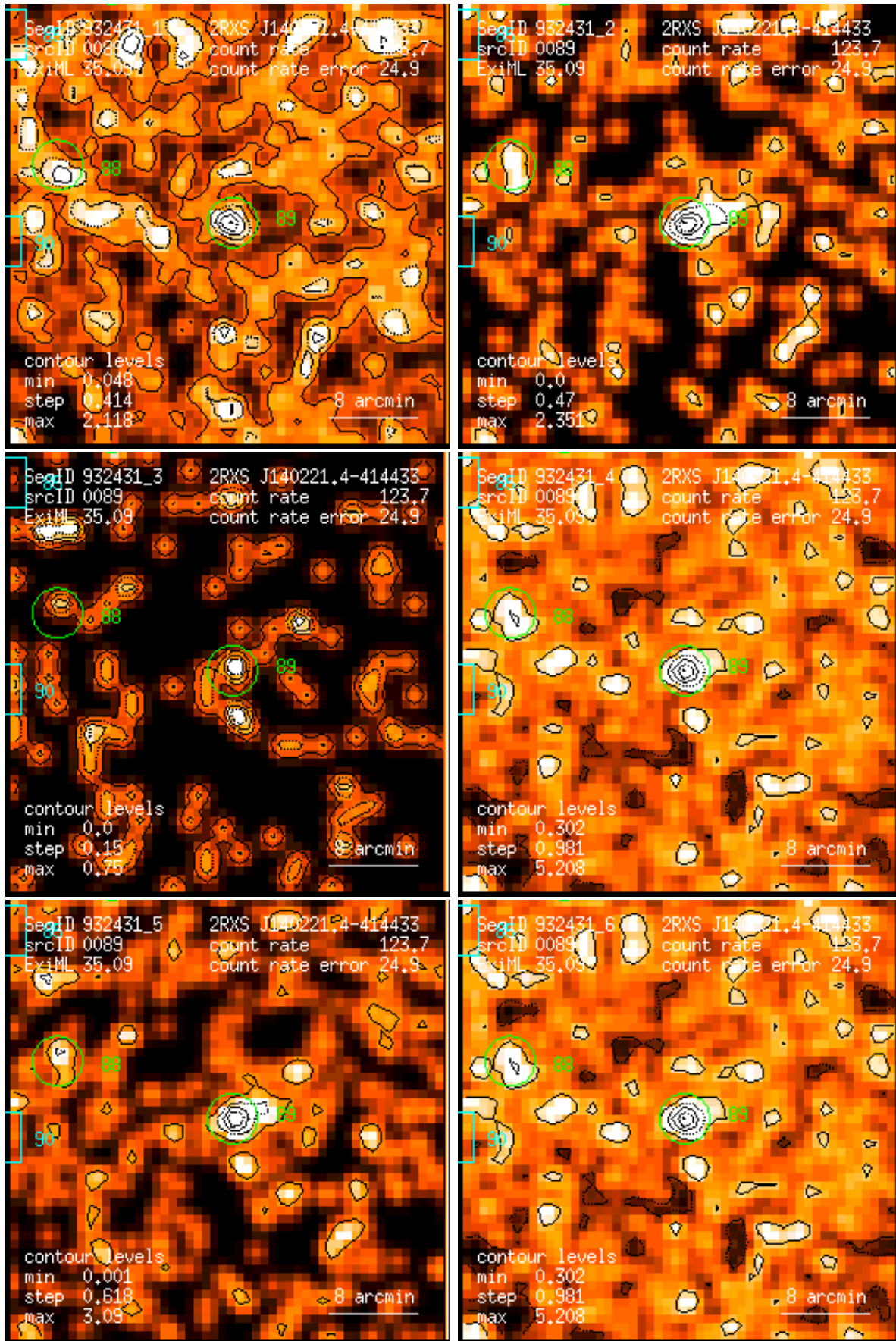
Figure 89: RASS 932431: detection 0089: band rate images, Gaussian filter: (1) PSPC channels 11 – 41, (2) 52 – 90, (3) 91 – 201, (4) 11 – 235, (5) 52 – 201, (6) 11 – 201. Broad band rates in counts/ks. Band rate contour levels in counts/ks/arcmin 2 .
